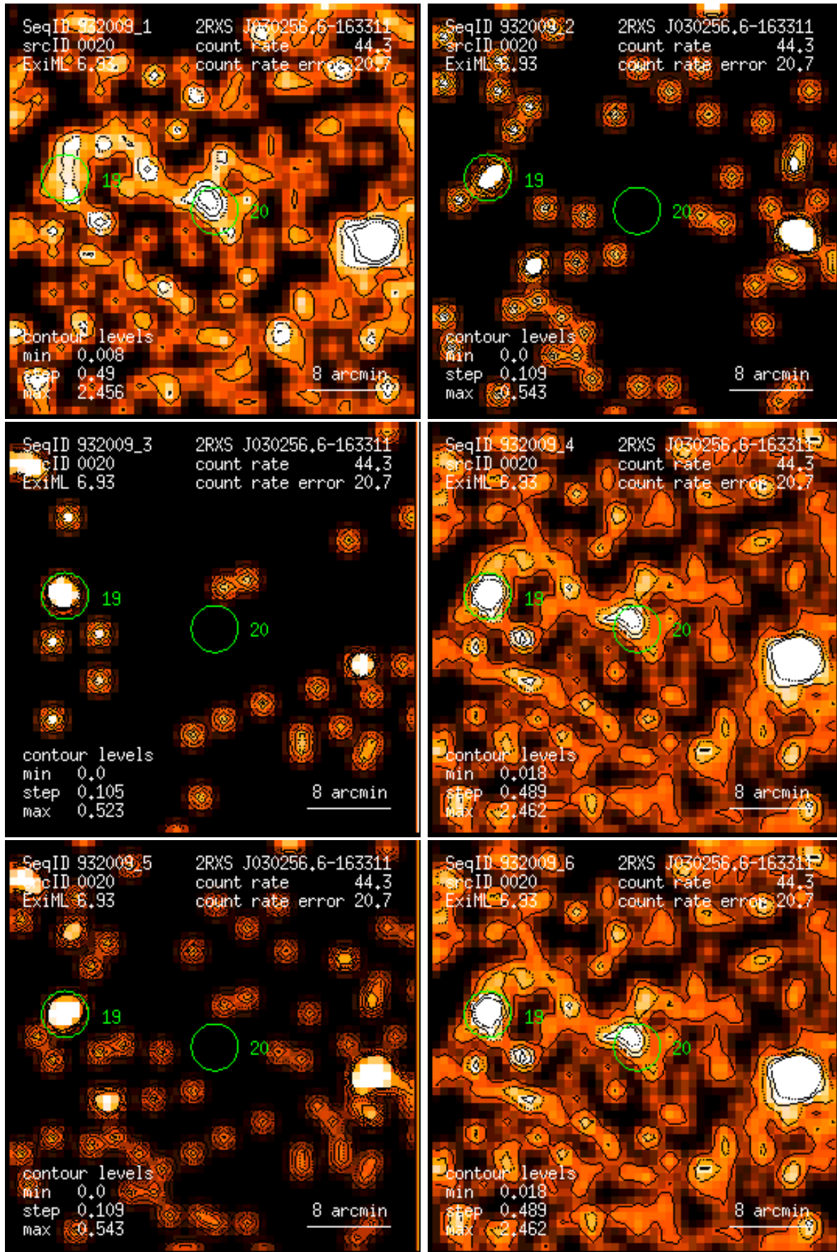
Figure 20: RASS 932009: detection 0020: band rate images, Gaussian filter: (1) PSPC channels 11 – 41, (2) 52 – 90, (3) 91 – 201, (4) 11 – 235, (5) 52 – 201, (6) 11 – 201. Broad band rates in counts/ks. Band rate contour levels in counts/ks/arcmin 2 .
