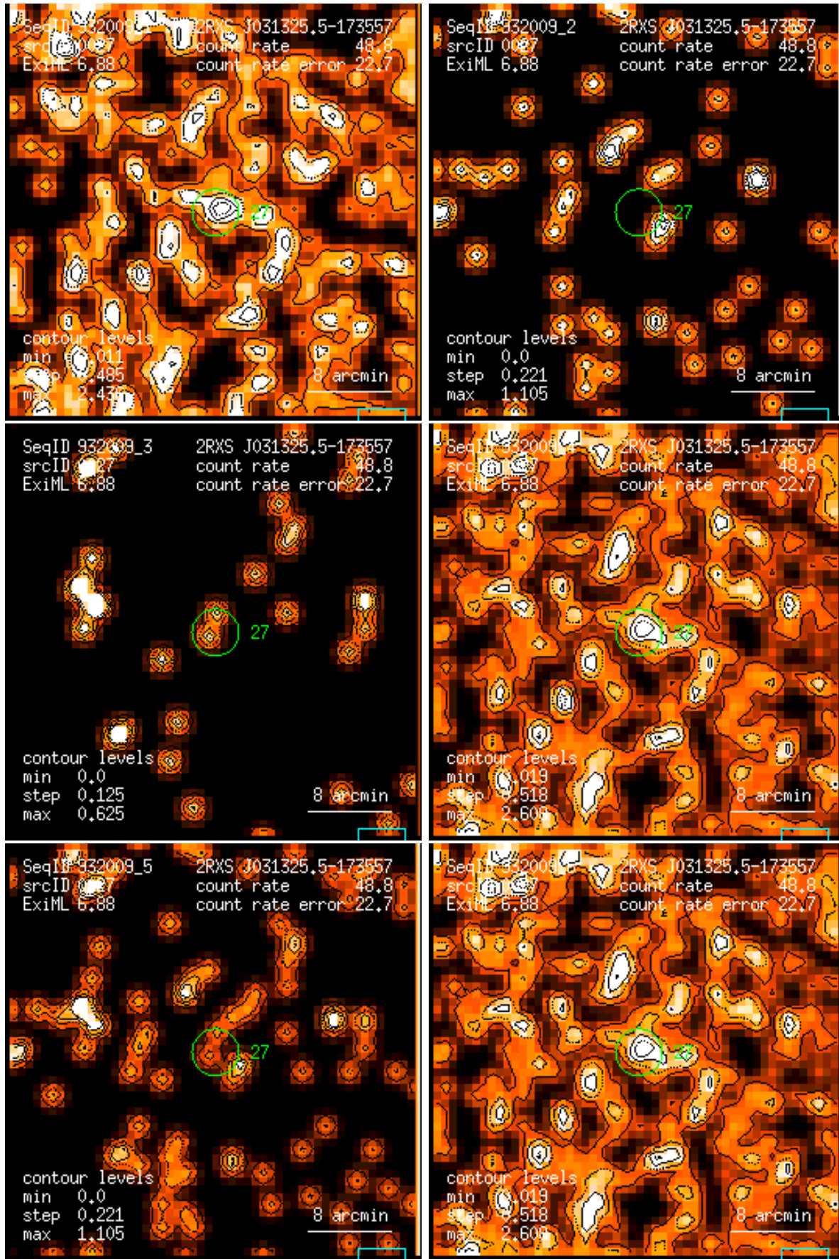
Figure 27: RASS 932009: detection 0027: band rate images, Gaussian filter: (1) PSPC channels 11 – 41, (2) 52 – 90, (3) 91 – 201, (4) 11 – 235, (5) 52 – 201, (6) 11 – 201. Broad band rates in counts/ks. Band rate contour levels in counts/ks/arcmin 2 .
