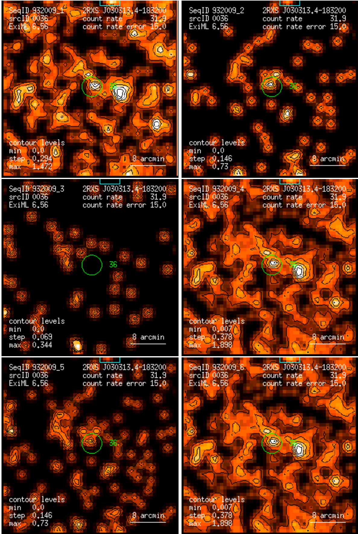
Figure 36: RASS 932009: detection 0036: band rate images, Gaussian filter: (1) PSPC channels 11 – 41, (2) 52 – 90, (3) 91 – 201, (4) 11 – 235, (5) 52 – 201, (6) 11 – 201. Broad band rates in counts/ks. Band rate contour levels in counts/ks/arcmin 2 .
