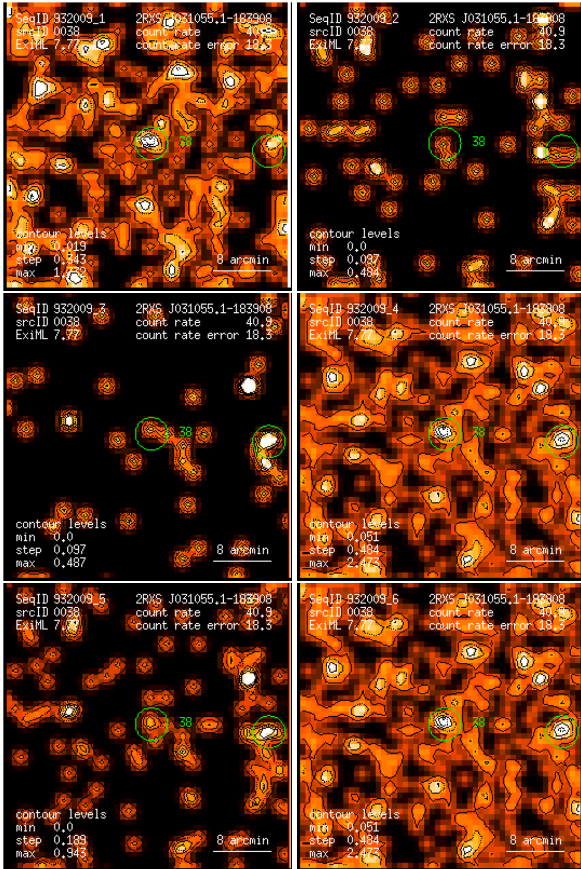
Figure 38: RASS 932009: detection 0038: band rate images, Gaussian filter: (1) PSPC channels 11 – 41, (2) 52 – 90, (3) 91 – 201, (4) 11 – 235, (5) 52 – 201, (6) 11 – 201. Broad band rates in counts/ks. Band rate contour levels in counts/ks/arcmin 2 .
