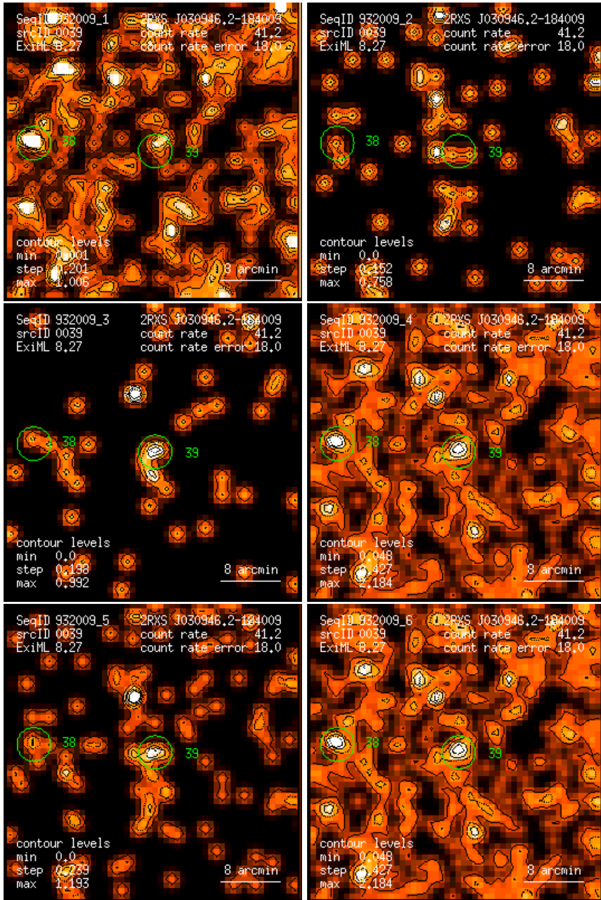
Figure 39: RASS 932009: detection 0039: band rate images, Gaussian filter: (1) PSPC channels 11 – 41, (2) 52 – 90, (3) 91 – 201, (4) 11 – 235, (5) 52 – 201, (6) 11 – 201. Broad band rates in counts/ks. Band rate contour levels in counts/ks/arcmin 2 .
