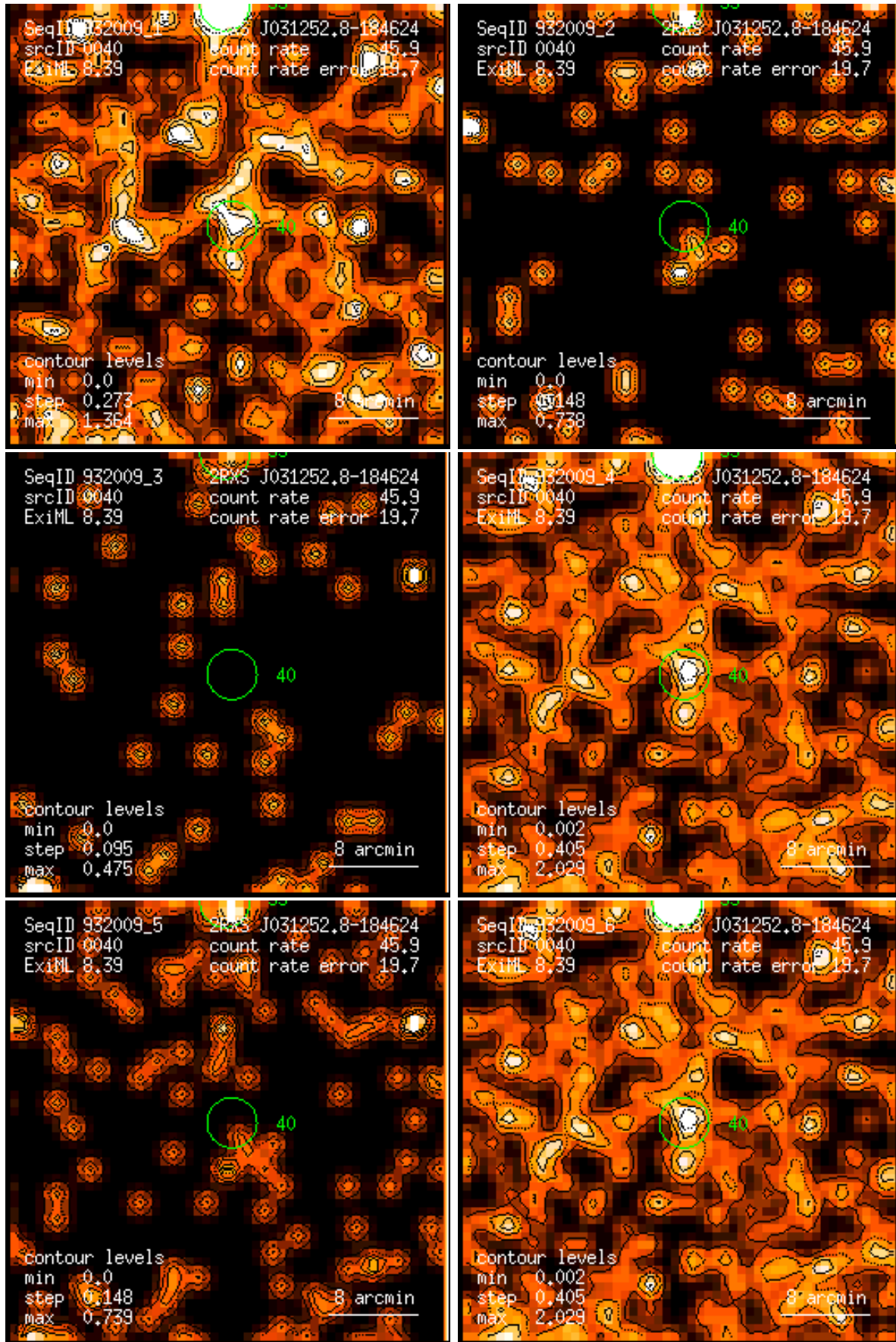
Figure 40: RASS 932009: detection 0040: band rate images, Gaussian filter: (1) PSPC channels 11 – 41, (2) 52 – 90, (3) 91 – 201, (4) 11 – 235, (5) 52 – 201, (6) 11 – 201. Broad band rates in counts/ks. Band rate contour levels in counts/ks/arcmin 2 .
