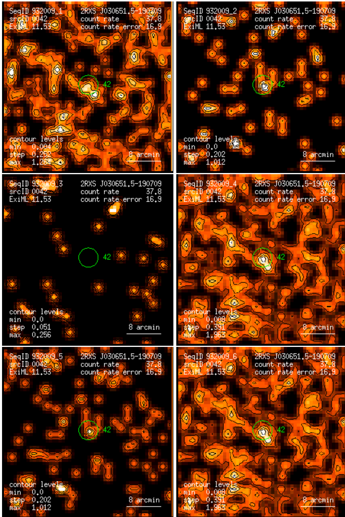
Figure 42: RASS 932009: detection 0042: band rate images, Gaussian filter: (1) PSPC channels 11 – 41, (2) 52 – 90, (3) 91 – 201, (4) 11 – 235, (5) 52 – 201, (6) 11 – 201. Broad band rates in counts/ks. Band rate contour levels in counts/ks/arcmin 2 .
