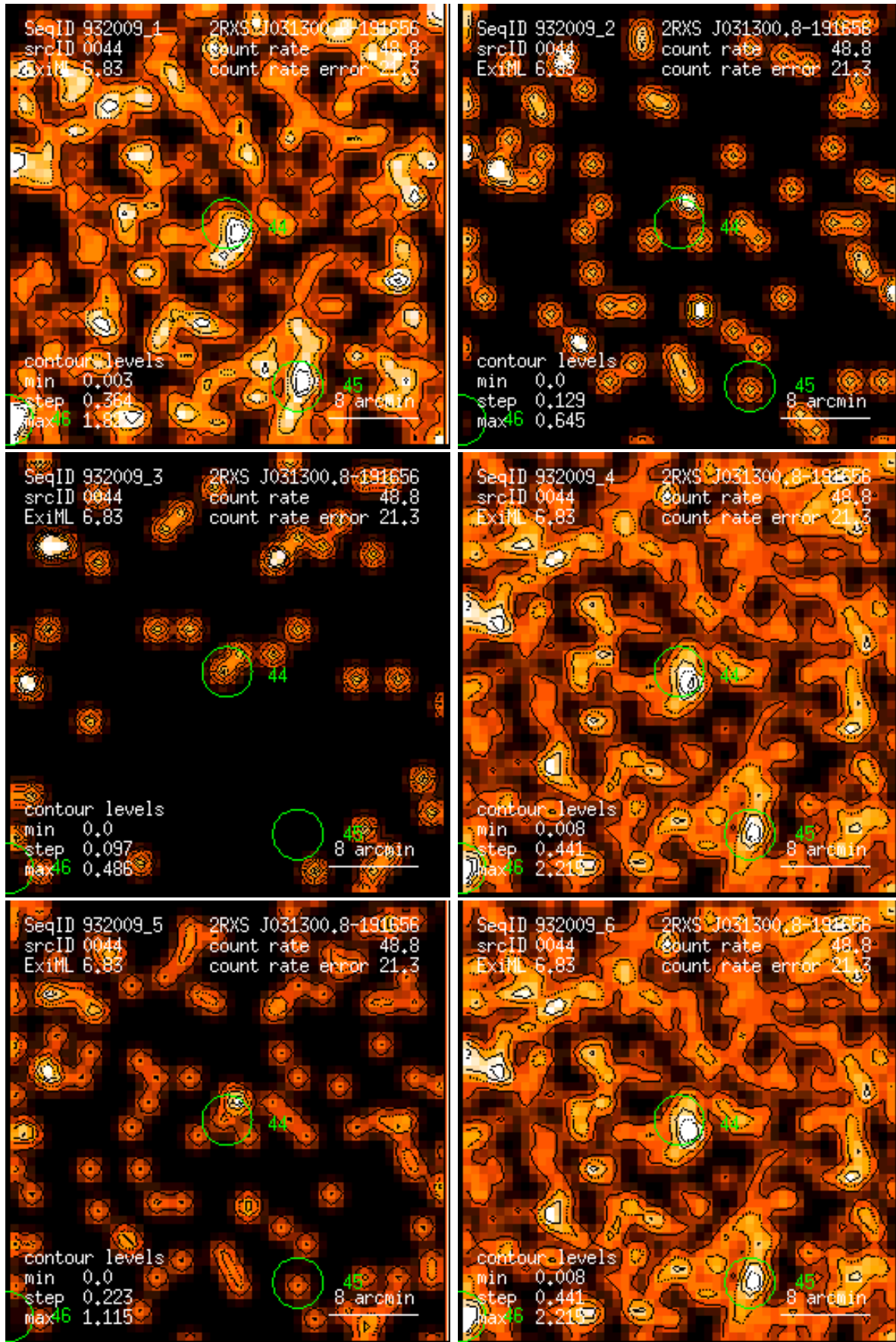
Figure 44: RASS 932009: detection 0044: band rate images, Gaussian filter: (1) PSPC channels 11 – 41, (2) 52 – 90, (3) 91 – 201, (4) 11 – 235, (5) 52 – 201, (6) 11 – 201. Broad band rates in counts/ks. Band rate contour levels in counts/ks/arcmin 2 .
