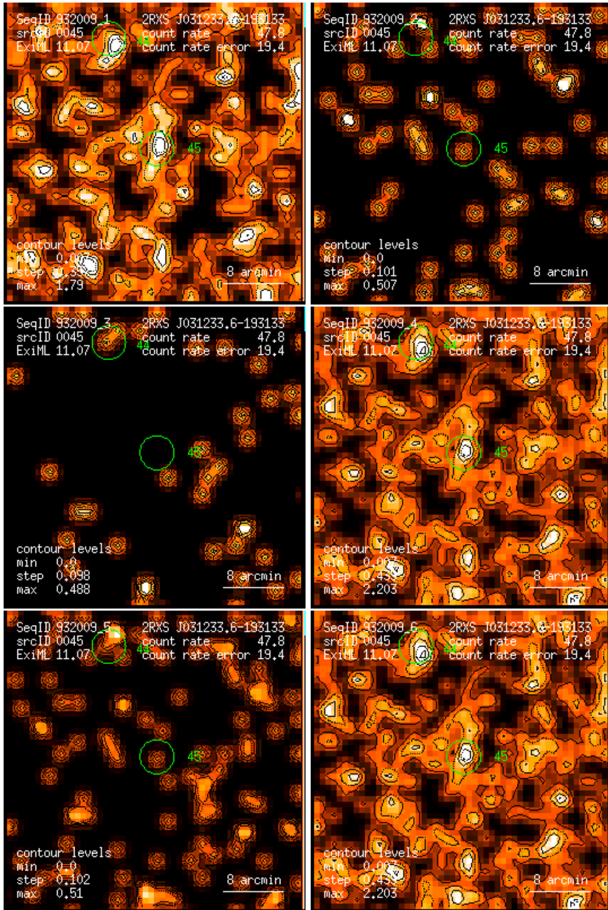
Figure 45: RASS 932009: detection 0045: band rate images, Gaussian filter: (1) PSPC channels 11 – 41, (2) 52 – 90, (3) 91 – 201, (4) 11 – 235, (5) 52 – 201, (6) 11 – 201. Broad band rates in counts/ks. Band rate contour levels in counts/ks/arcmin 2 .
