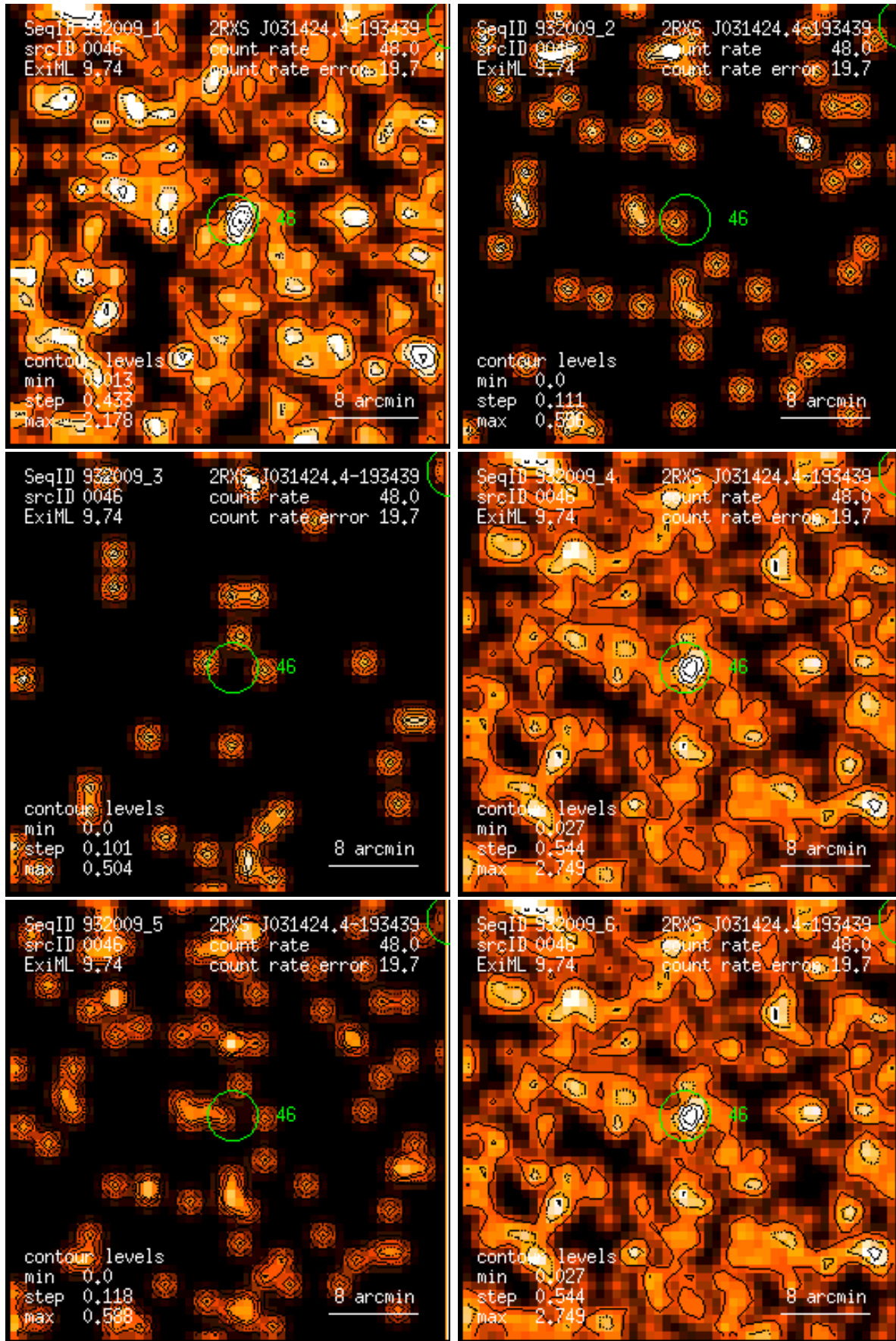
Figure 46: RASS 932009: detection 0046: band rate images, Gaussian filter: (1) PSPC channels 11 – 41, (2) 52 – 90, (3) 91 – 201, (4) 11 – 235, (5) 52 – 201, (6) 11 – 201. Broad band rates in counts/ks. Band rate contour levels in counts/ks/arcmin 2 .
