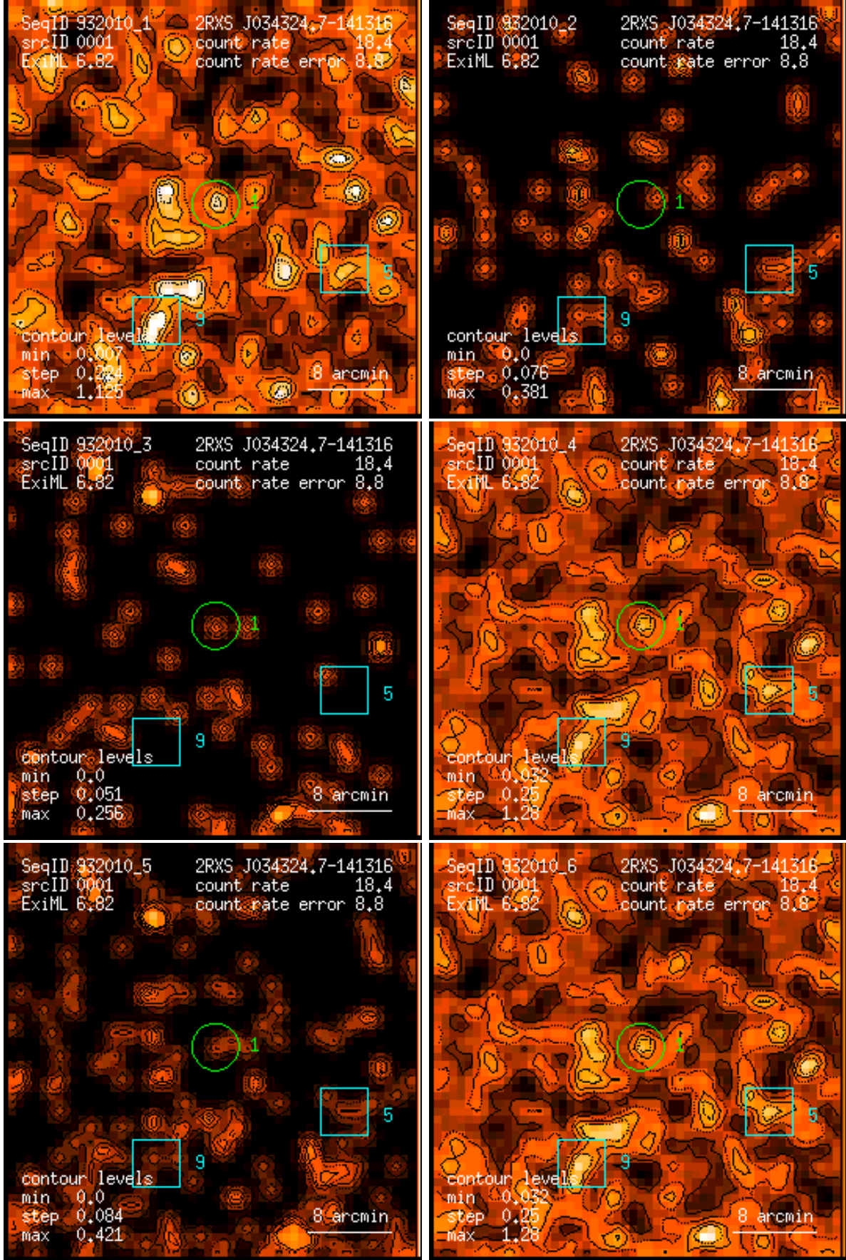
Figure 1: RASS 932010: detection 0001: band rate images, Gaussian filter: (1) PSPC channels 11 – 41, (2) 52 – 90, (3) 91 – 201, (4) 11 – 235, (5) 52 – 201, (6) 11 – 201. Broad band rates in counts/ks. Band rate contour levels in counts/ks/arcmin 2 .
