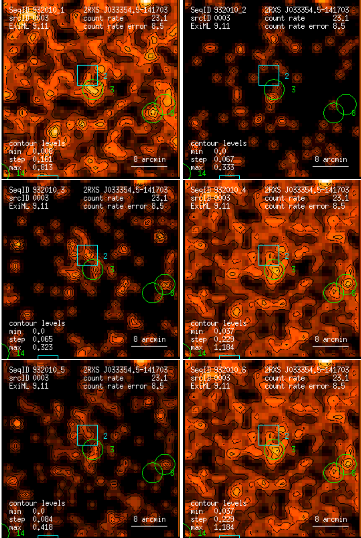
Figure 3: RASS 932010: detection 0003: band rate images, Gaussian filter: (1) PSPC channels 11 – 41, (2) 52 – 90, (3) 91 – 201, (4) 11 – 235, (5) 52 – 201, (6) 11 – 201. Broad band rates in counts/ks. Band rate contour levels in counts/ks/arcmin 2 .
