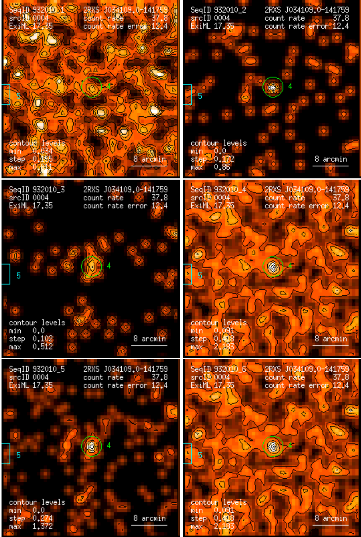
Figure 4: RASS 932010: detection 0004: band rate images, Gaussian filter: (1) PSPC channels 11 – 41, (2) 52 – 90, (3) 91 – 201, (4) 11 – 235, (5) 52 – 201, (6) 11 – 201. Broad band rates in counts/ks. Band rate contour levels in counts/ks/arcmin 2 .
