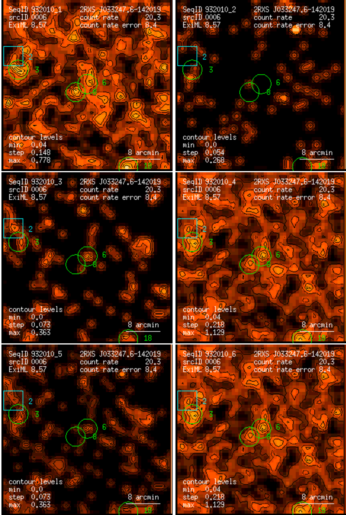
Figure 6: RASS 932010: detection 0006: band rate images, Gaussian filter: (1) PSPC channels 11 – 41, (2) 52 – 90, (3) 91 – 201, (4) 11 – 235, (5) 52 – 201, (6) 11 – 201. Broad band rates in counts/ks. Band rate contour levels in counts/ks/arcmin 2 .
