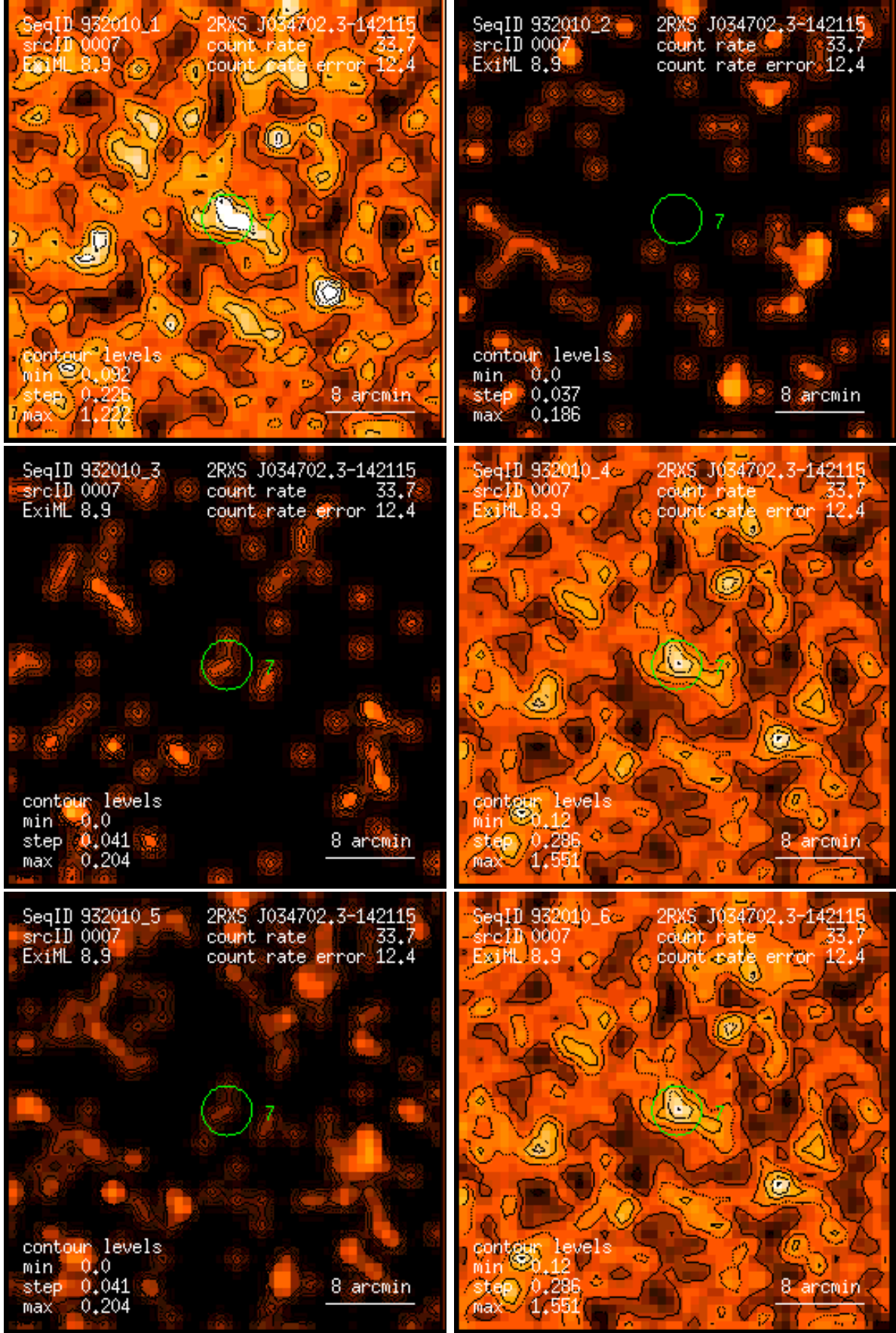
Figure 7: RASS 932010: detection 0007: band rate images, Gaussian filter: (1) PSPC channels 11 – 41, (2) 52 – 90, (3) 91 – 201, (4) 11 – 235, (5) 52 – 201, (6) 11 – 201. Broad band rates in counts/ks. Band rate contour levels in counts/ks/arcmin 2 .
