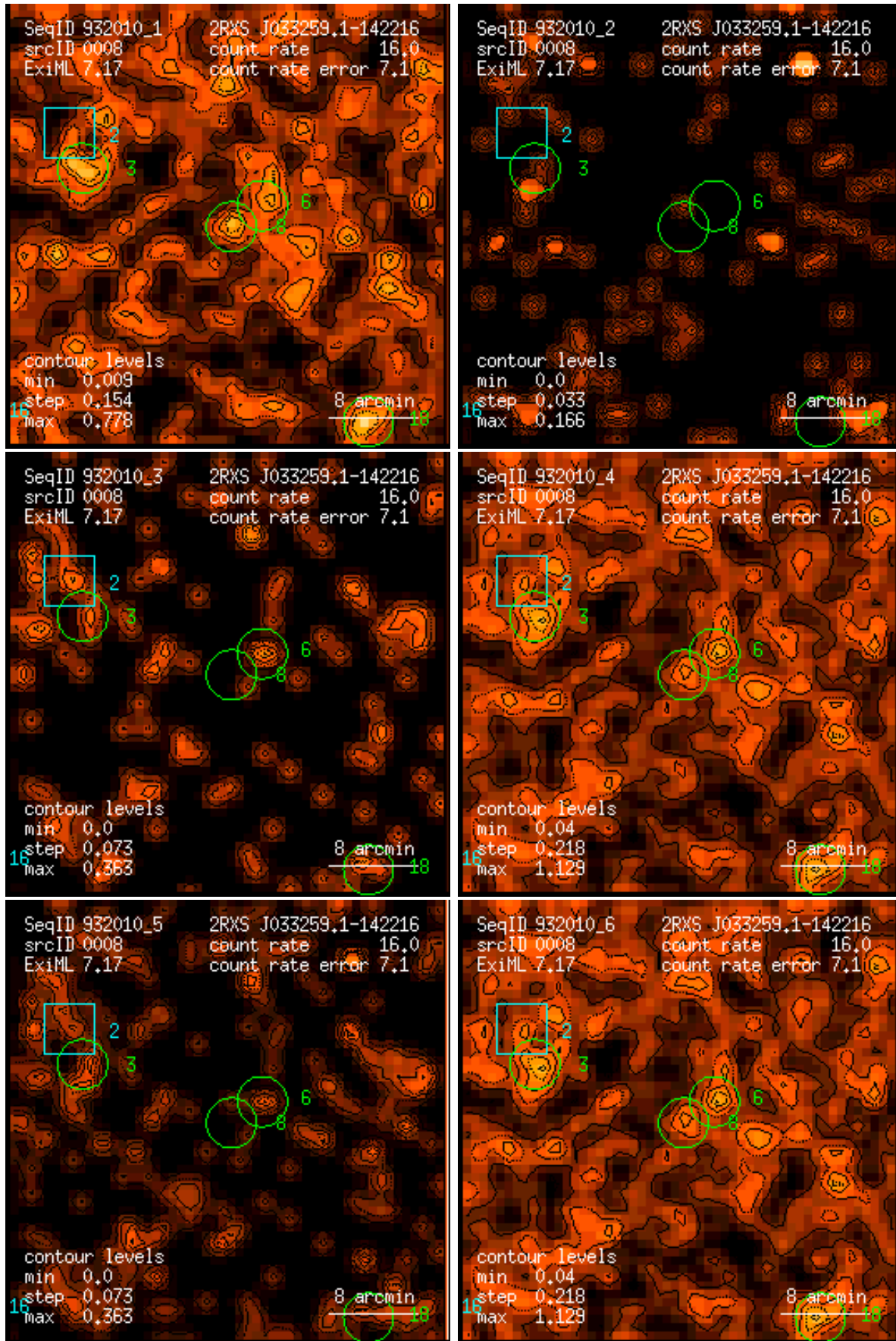
Figure 8: RASS 932010: detection 0008: band rate images, Gaussian filter: (1) PSPC channels 11 – 41, (2) 52 – 90, (3) 91 – 201, (4) 11 – 235, (5) 52 – 201, (6) 11 – 201. Broad band rates in counts/ks. Band rate contour levels in counts/ks/arcmin 2 .
