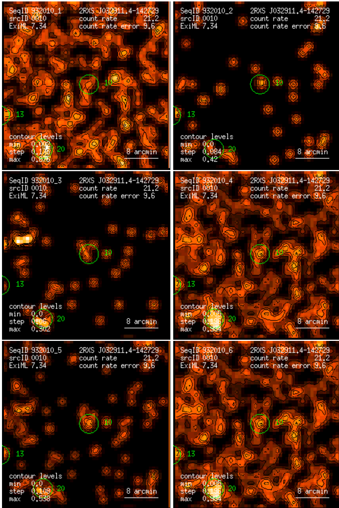
Figure 10: RASS 932010: detection 0010: band rate images, Gaussian filter: (1) PSPC channels 11 – 41, (2) 52 – 90, (3) 91 – 201, (4) 11 – 235, (5) 52 – 201, (6) 11 – 201. Broad band rates in counts/ks. Band rate contour levels in counts/ks/arcmin 2 .
