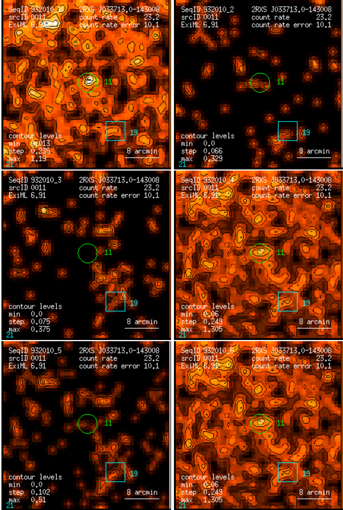
Figure 11: RASS 932010: detection 0011: band rate images, Gaussian filter: (1) PSPC channels 11 – 41, (2) 52 – 90, (3) 91 – 201, (4) 11 – 235, (5) 52 – 201, (6) 11 – 201. Broad band rates in counts/ks. Band rate contour levels in counts/ks/arcmin 2 .
