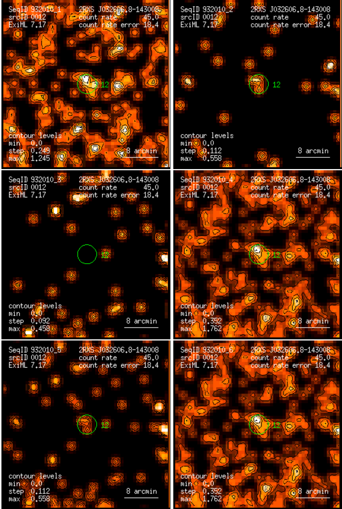
Figure 12: RASS 932010: detection 0012: band rate images, Gaussian filter: (1) PSPC channels 11 – 41, (2) 52 – 90, (3) 91 – 201, (4) 11 – 235, (5) 52 – 201, (6) 11 – 201. Broad band rates in counts/ks. Band rate contour levels in counts/ks/arcmin 2 .
