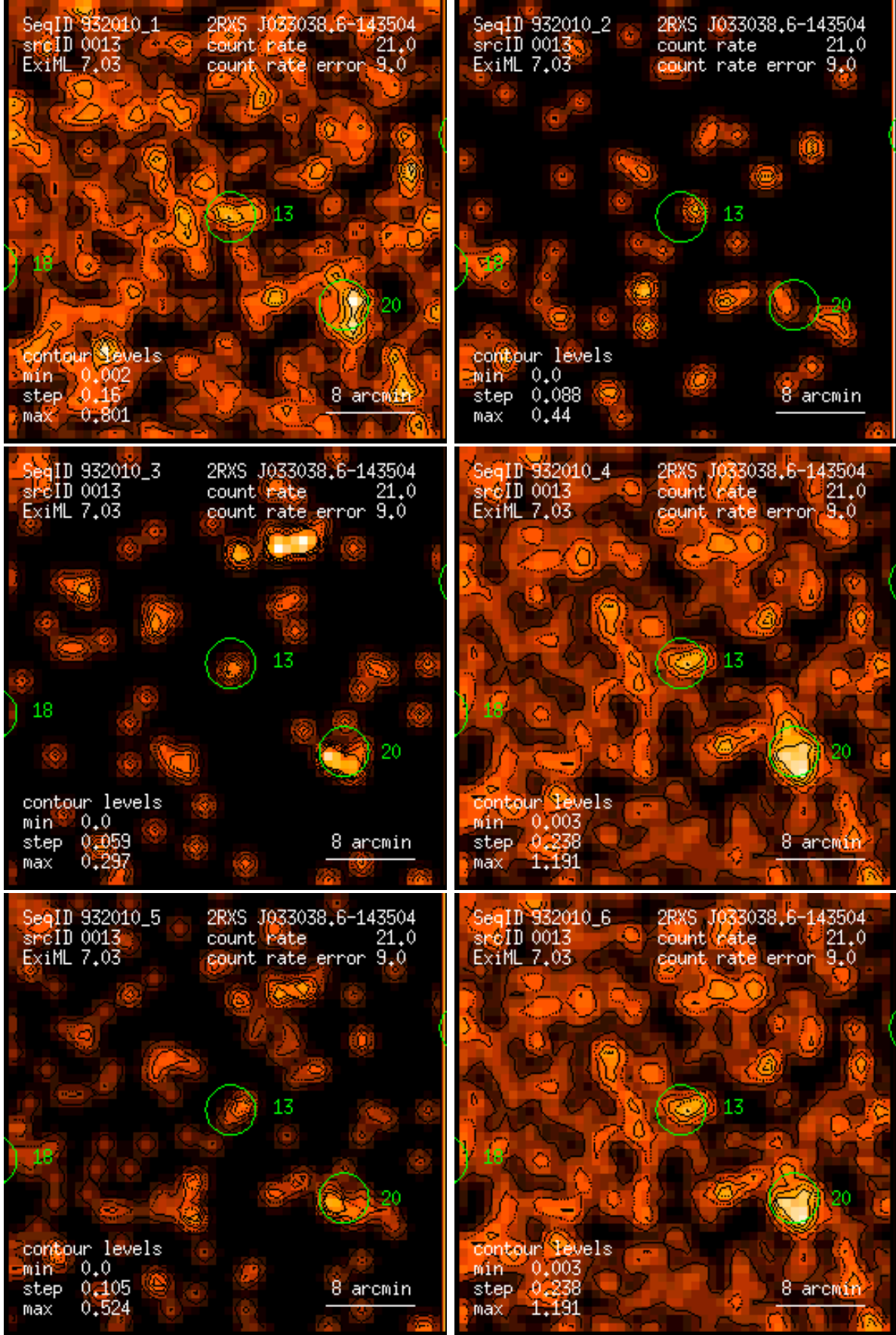
Figure 13: RASS 932010: detection 0013: band rate images, Gaussian filter: (1) PSPC channels 11 – 41, (2) 52 – 90, (3) 91 – 201, (4) 11 – 235, (5) 52 – 201, (6) 11 – 201. Broad band rates in counts/ks. Band rate contour levels in counts/ks/arcmin 2 .
