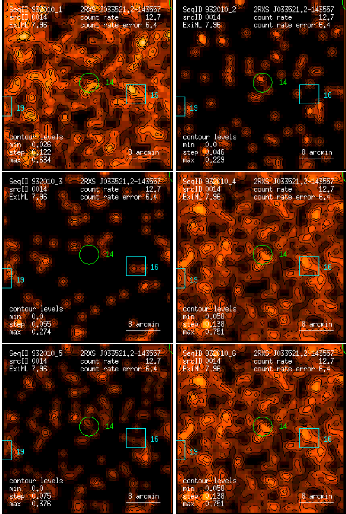
Figure 14: RASS 932010: detection 0014: band rate images, Gaussian filter: (1) PSPC channels 11 – 41, (2) 52 – 90, (3) 91 – 201, (4) 11 – 235, (5) 52 – 201, (6) 11 – 201. Broad band rates in counts/ks. Band rate contour levels in counts/ks/arcmin 2 .
