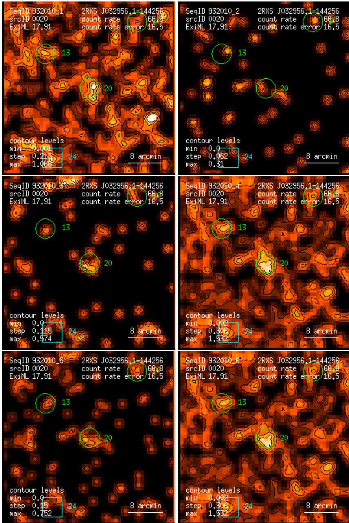
Figure 20: RASS 932010: detection 0020: band rate images, Gaussian filter: (1) PSPC channels 11 – 41, (2) 52 – 90, (3) 91 – 201, (4) 11 – 235, (5) 52 – 201, (6) 11 – 201. Broad band rates in counts/ks. Band rate contour levels in counts/ks/arcmin 2 .
