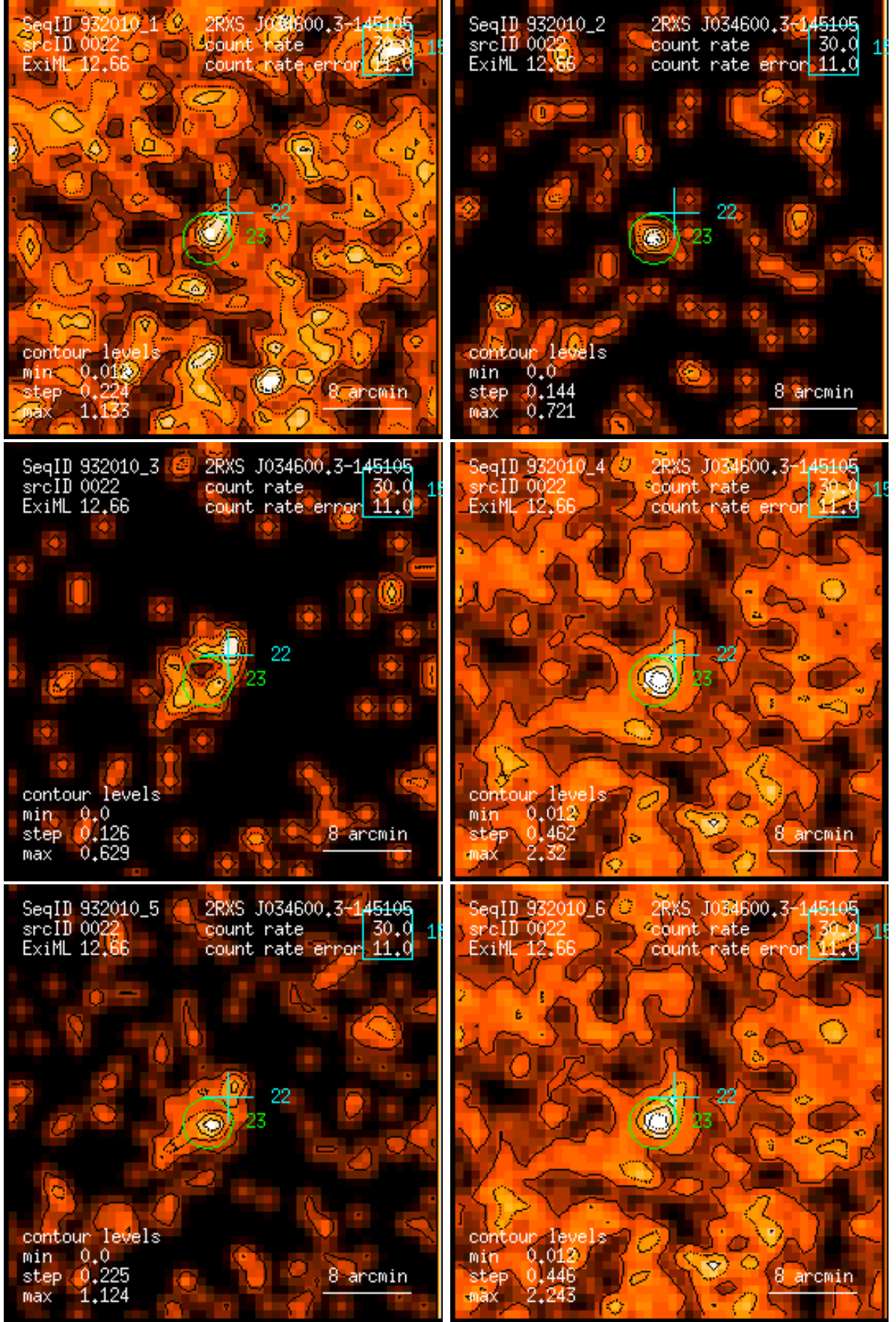
Figure 22: RASS 932010: detection 0022: band rate images, Gaussian filter: (1) PSPC channels 11 – 41, (2) 52 – 90, (3) 91 – 201, (4) 11 – 235, (5) 52 – 201, (6) 11 – 201. Broad band rates in counts/ks. Band rate contour levels in counts/ks/arcmin 2 .
