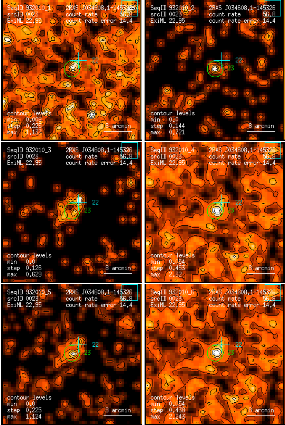
Figure 23: RASS 932010: detection 0023: band rate images, Gaussian filter: (1) PSPC channels 11 – 41, (2) 52 – 90, (3) 91 – 201, (4) 11 – 235, (5) 52 – 201, (6) 11 – 201. Broad band rates in counts/ks. Band rate contour levels in counts/ks/arcmin 2 .
