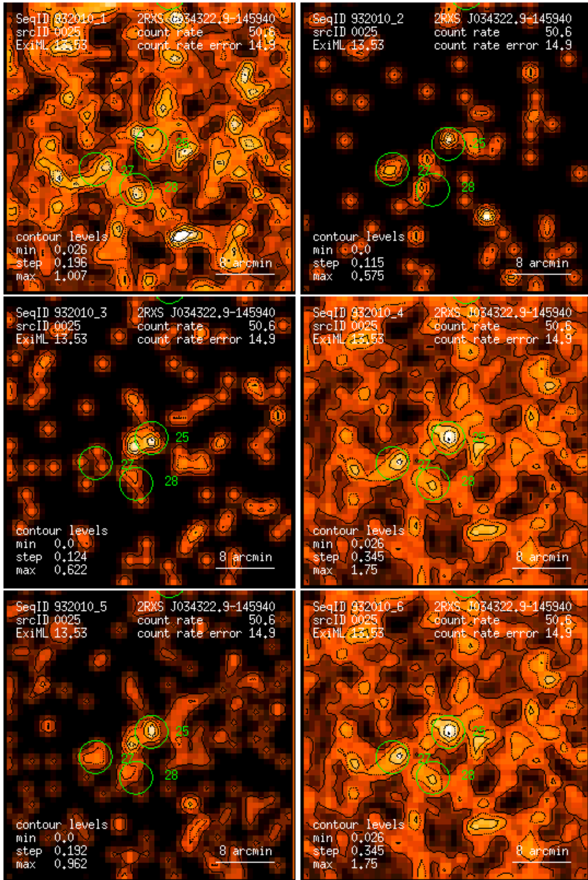
Figure 25: RASS 932010: detection 0025: band rate images, Gaussian filter: (1) PSPC channels 11 – 41, (2) 52 – 90, (3) 91 – 201, (4) 11 – 235, (5) 52 – 201, (6) 11 – 201. Broad band rates in counts/ks. Band rate contour levels in counts/ks/arcmin 2 .
