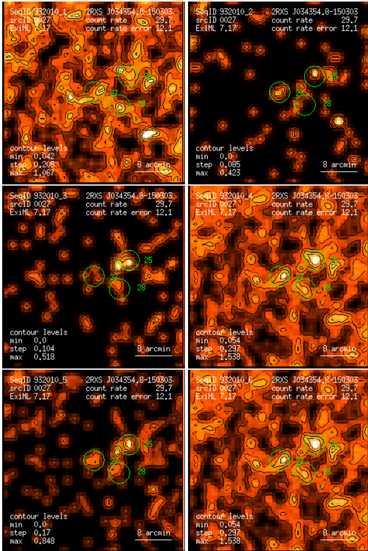
Figure 27: RASS 932010: detection 0027: band rate images, Gaussian filter: (1) PSPC channels 11 – 41, (2) 52 – 90, (3) 91 – 201, (4) 11 – 235, (5) 52 – 201, (6) 11 – 201. Broad band rates in counts/ks. Band rate contour levels in counts/ks/arcmin 2 .
