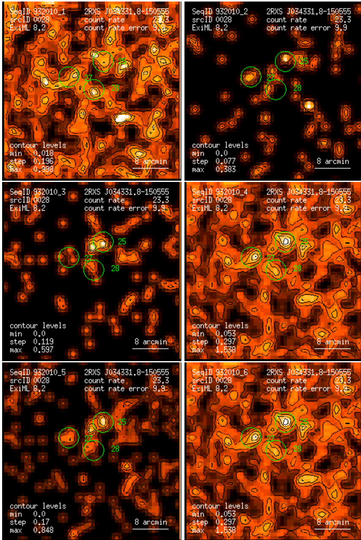
Figure 28: RASS 932010: detection 0028: band rate images, Gaussian filter: (1) PSPC channels 11 – 41, (2) 52 – 90, (3) 91 – 201, (4) 11 – 235, (5) 52 – 201, (6) 11 – 201. Broad band rates in counts/ks. Band rate contour levels in counts/ks/arcmin 2 .
