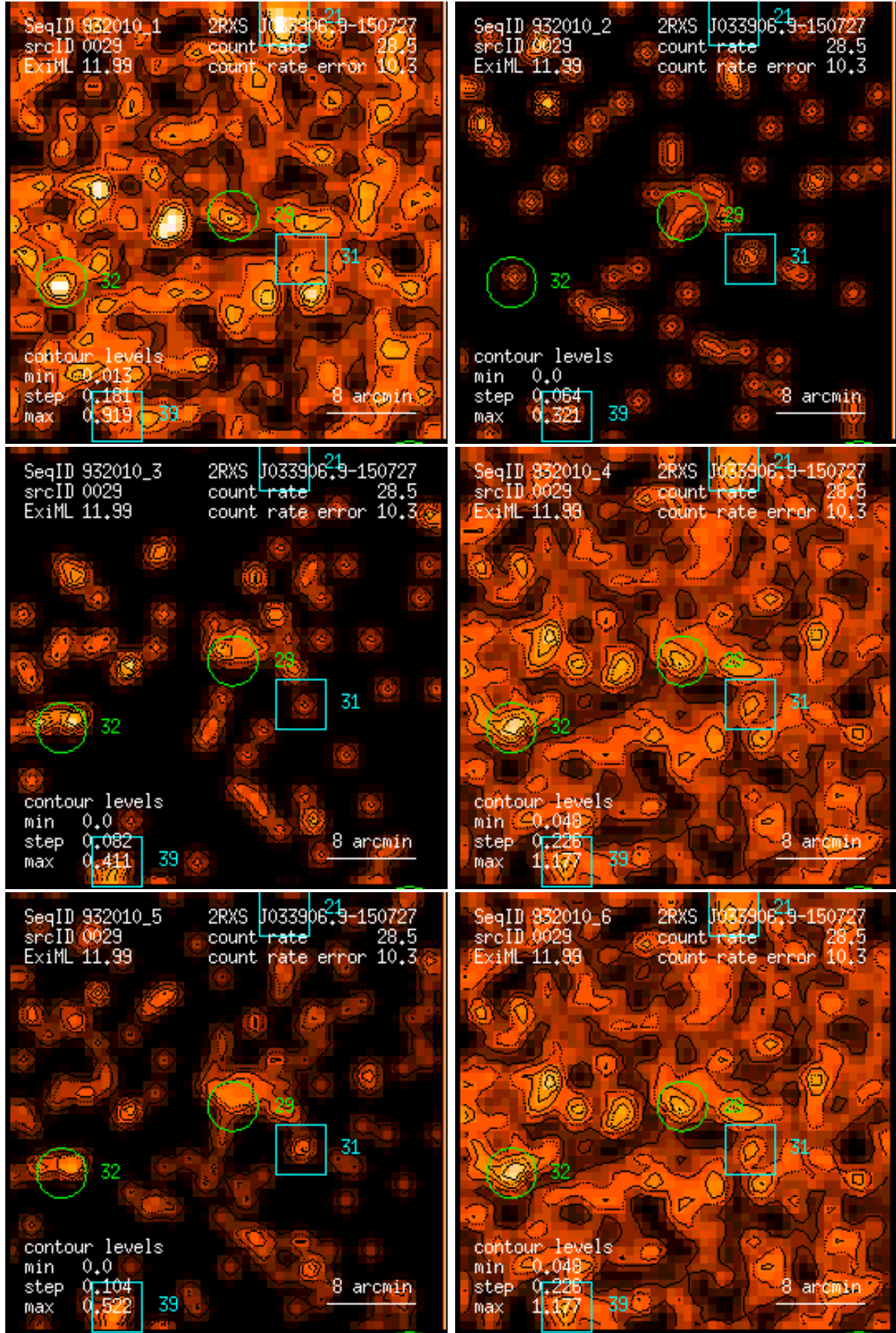
Figure 29: RASS 932010: detection 0029: band rate images, Gaussian filter: (1) PSPC channels 11 – 41, (2) 52 – 90, (3) 91 – 201, (4) 11 – 235, (5) 52 – 201, (6) 11 – 201. Broad band rates in counts/ks. Band rate contour levels in counts/ks/arcmin 2 .
