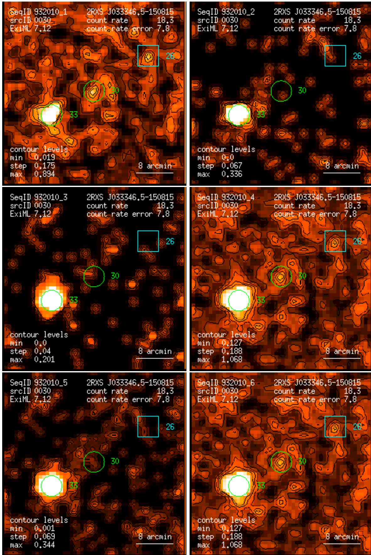
Figure 30: RASS 932010: detection 0030: band rate images, Gaussian filter: (1) PSPC channels 11 – 41, (2) 52 – 90, (3) 91 – 201, (4) 11 – 235, (5) 52 – 201, (6) 11 – 201. Broad band rates in counts/ks. Band rate contour levels in counts/ks/arcmin 2 .
