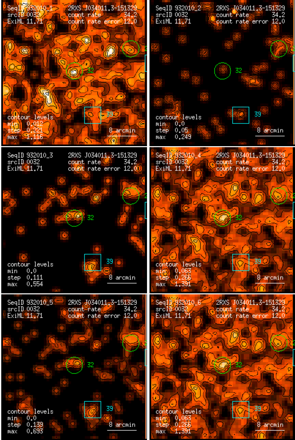
Figure 32: RASS 932010: detection 0032: band rate images, Gaussian filter: (1) PSPC channels 11 – 41, (2) 52 – 90, (3) 91 – 201, (4) 11 – 235, (5) 52 – 201, (6) 11 – 201. Broad band rates in counts/ks. Band rate contour levels in counts/ks/arcmin 2 .
