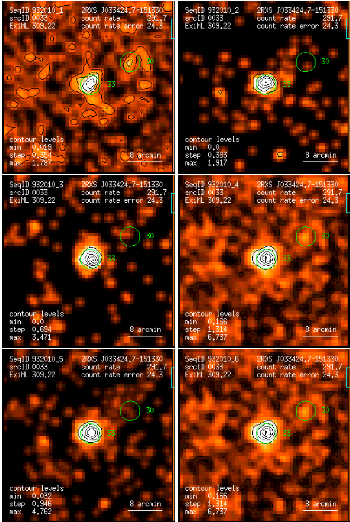
Figure 33: RASS 932010: detection 0033: band rate images, Gaussian filter: (1) PSPC channels 11 – 41, (2) 52 – 90, (3) 91 – 201, (4) 11 – 235, (5) 52 – 201, (6) 11 – 201. Broad band rates in counts/ks. Band rate contour levels in counts/ks/arcmin 2 .
