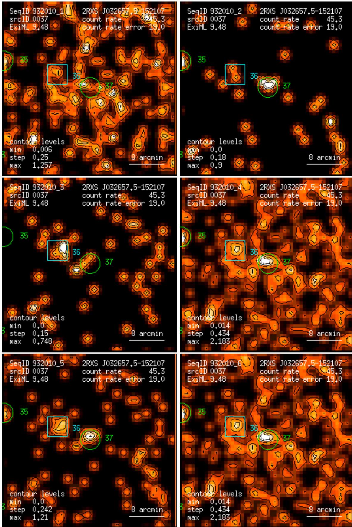
Figure 37: RASS 932010: detection 0037: band rate images, Gaussian filter: (1) PSPC channels 11 – 41, (2) 52 – 90, (3) 91 – 201, (4) 11 – 235, (5) 52 – 201, (6) 11 – 201. Broad band rates in counts/ks. Band rate contour levels in counts/ks/arcmin 2 .
