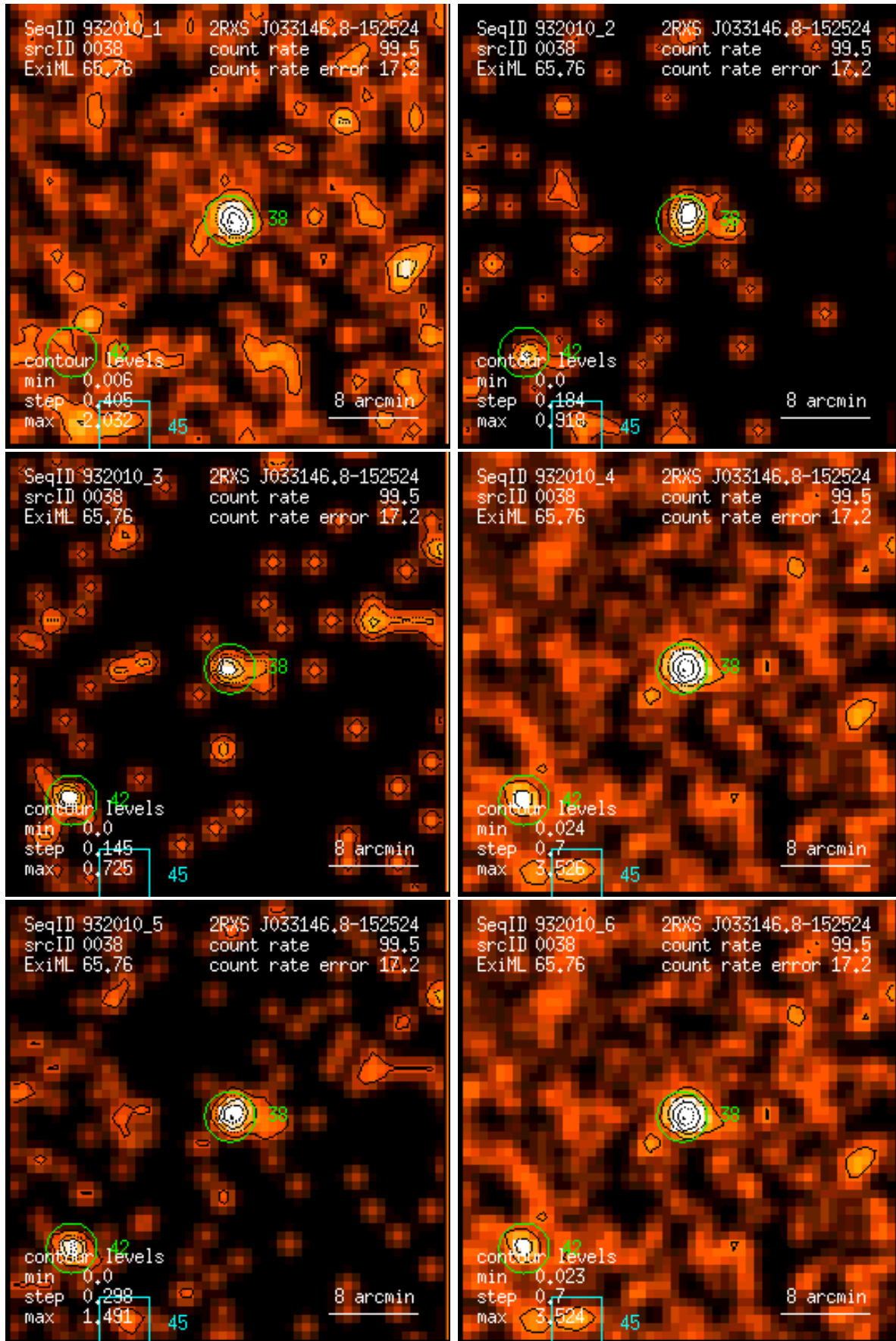
Figure 38: RASS 932010: detection 0038: band rate images, Gaussian filter: (1) PSPC channels 11 – 41, (2) 52 – 90, (3) 91 – 201, (4) 11 – 235, (5) 52 – 201, (6) 11 – 201. Broad band rates in counts/ks. Band rate contour levels in counts/ks/arcmin 2 .
