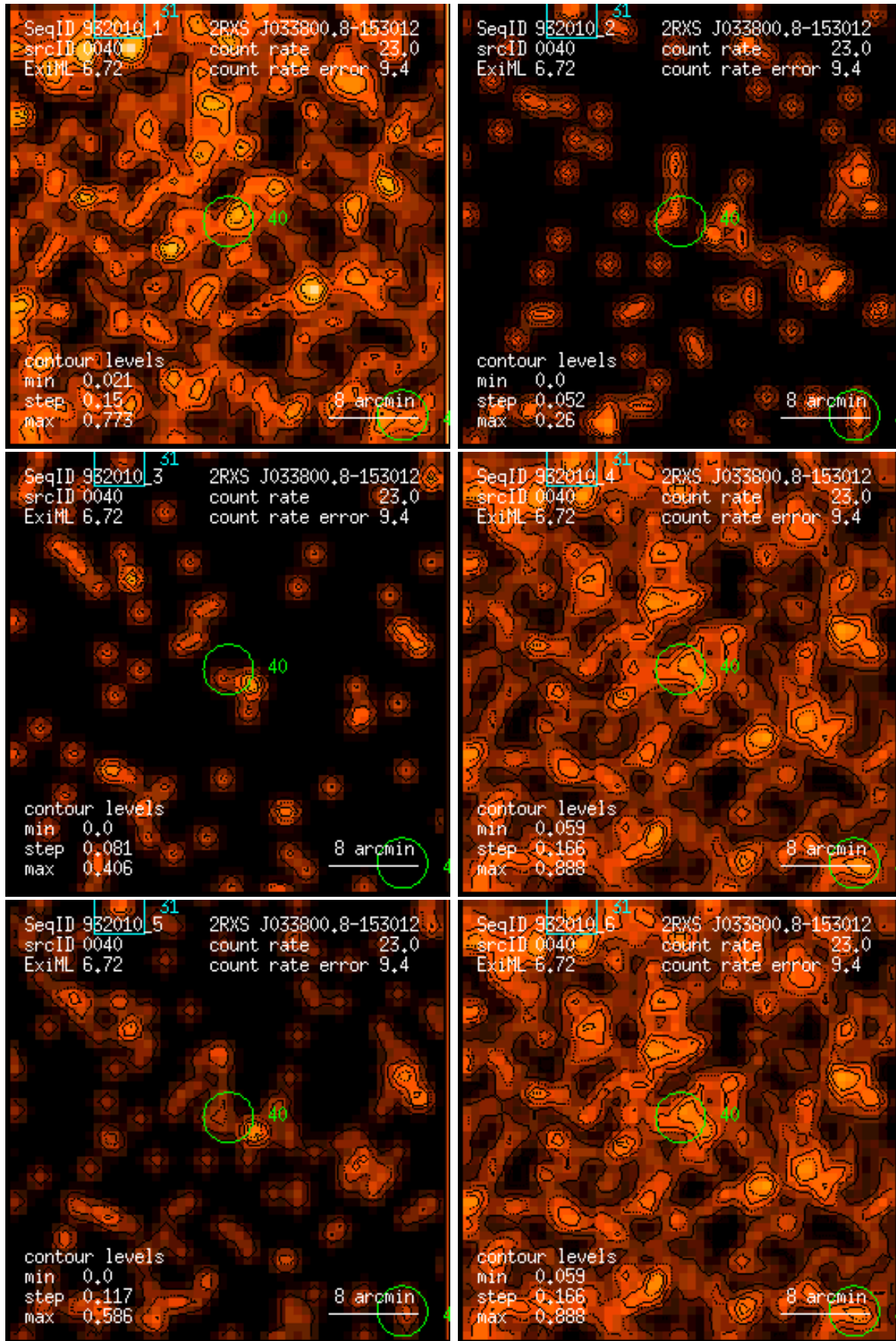
Figure 40: RASS 932010: detection 0040: band rate images, Gaussian filter: (1) PSPC channels 11 – 41, (2) 52 – 90, (3) 91 – 201, (4) 11 – 235, (5) 52 – 201, (6) 11 – 201. Broad band rates in counts/ks. Band rate contour levels in counts/ks/arcmin 2 .
