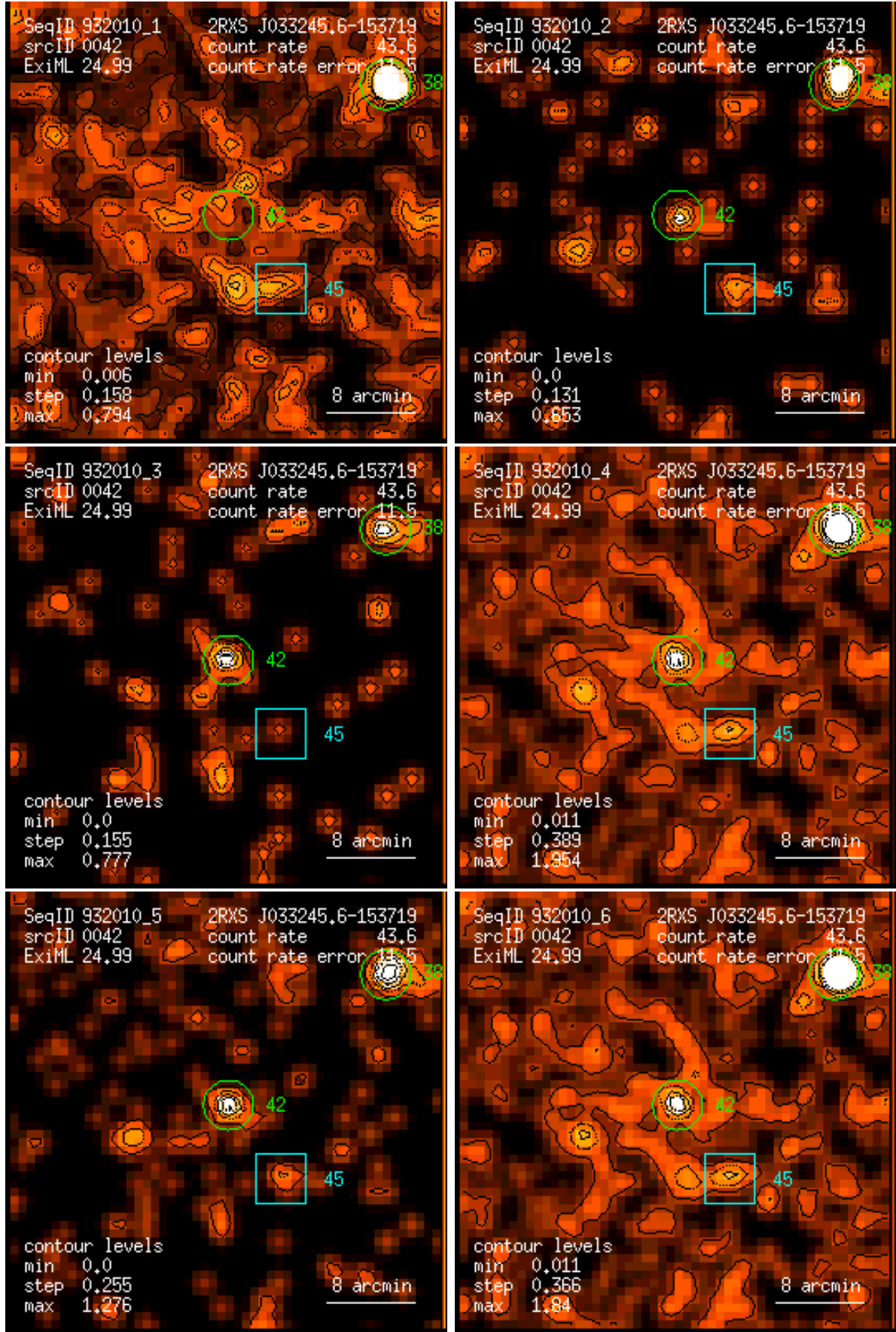
Figure 42: RASS 932010: detection 0042: band rate images, Gaussian filter: (1) PSPC channels 11 – 41, (2) 52 – 90, (3) 91 – 201, (4) 11 – 235, (5) 52 – 201, (6) 11 – 201. Broad band rates in counts/ks. Band rate contour levels in counts/ks/arcmin 2 .
