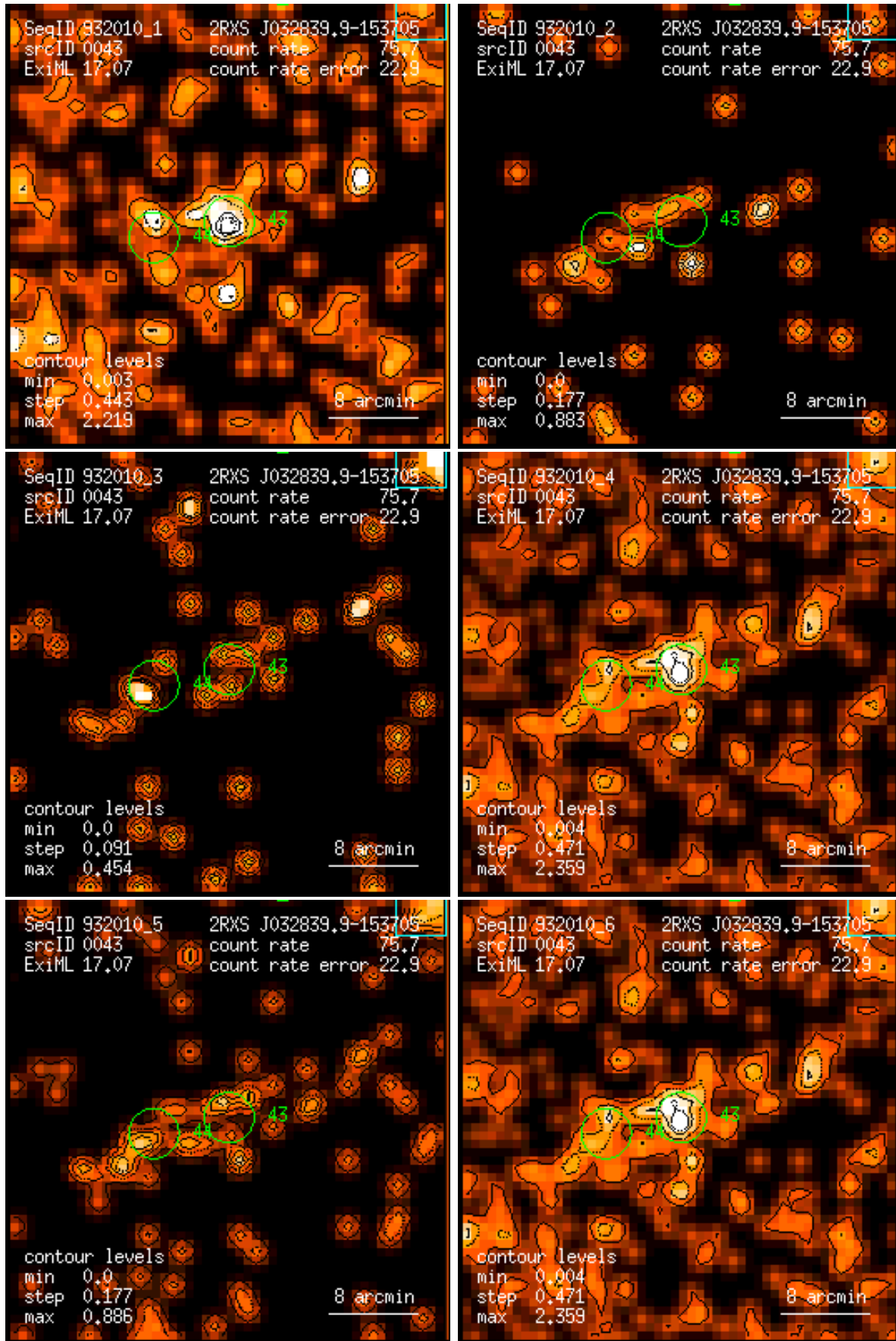
Figure 43: RASS 932010: detection 0043: band rate images, Gaussian filter: (1) PSPC channels 11 – 41, (2) 52 – 90, (3) 91 – 201, (4) 11 – 235, (5) 52 – 201, (6) 11 – 201. Broad band rates in counts/ks. Band rate contour levels in counts/ks/arcmin 2 .
