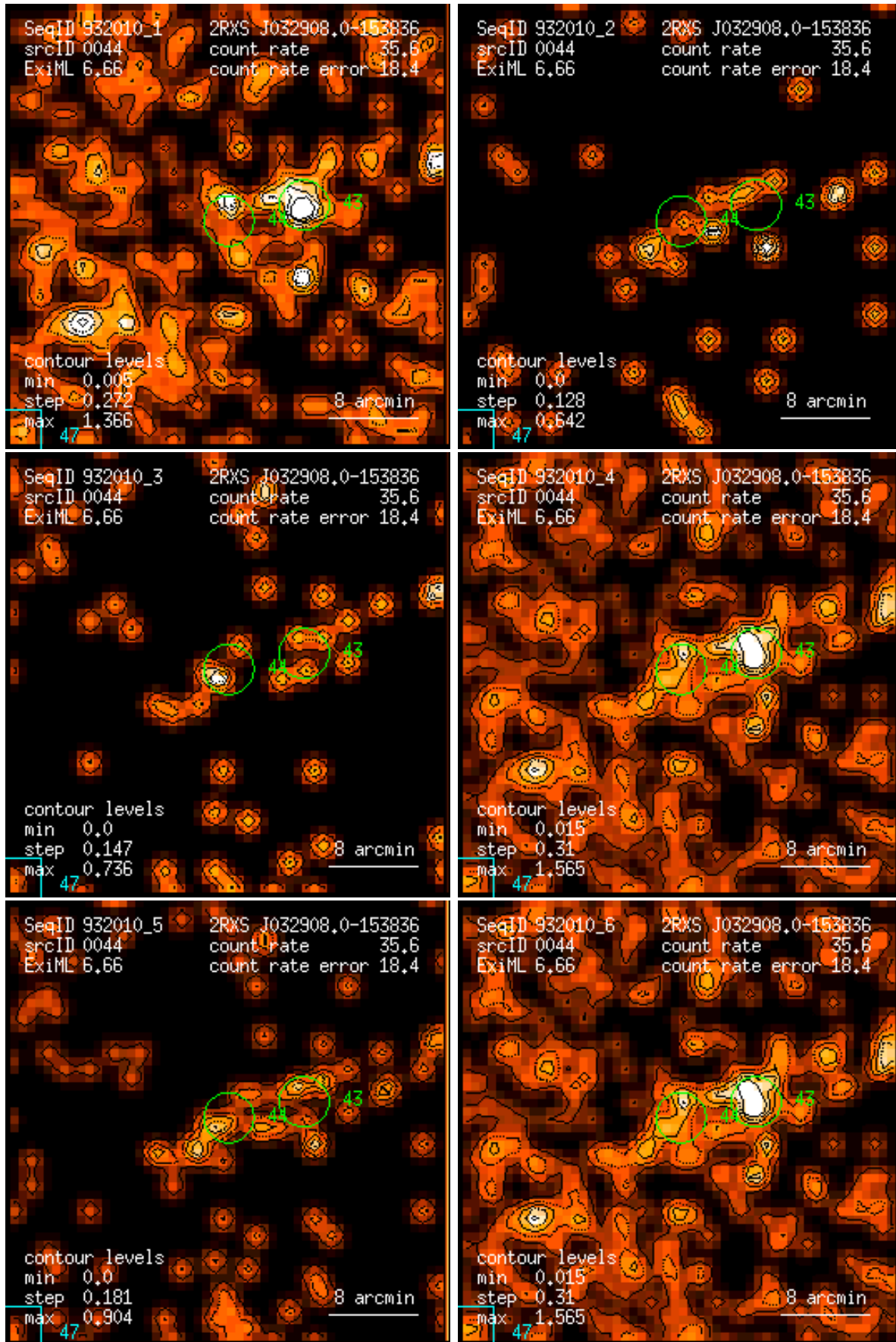
Figure 44: RASS 932010: detection 0044: band rate images, Gaussian filter: (1) PSPC channels 11 – 41, (2) 52 – 90, (3) 91 – 201, (4) 11 – 235, (5) 52 – 201, (6) 11 – 201. Broad band rates in counts/ks. Band rate contour levels in counts/ks/arcmin 2 .
