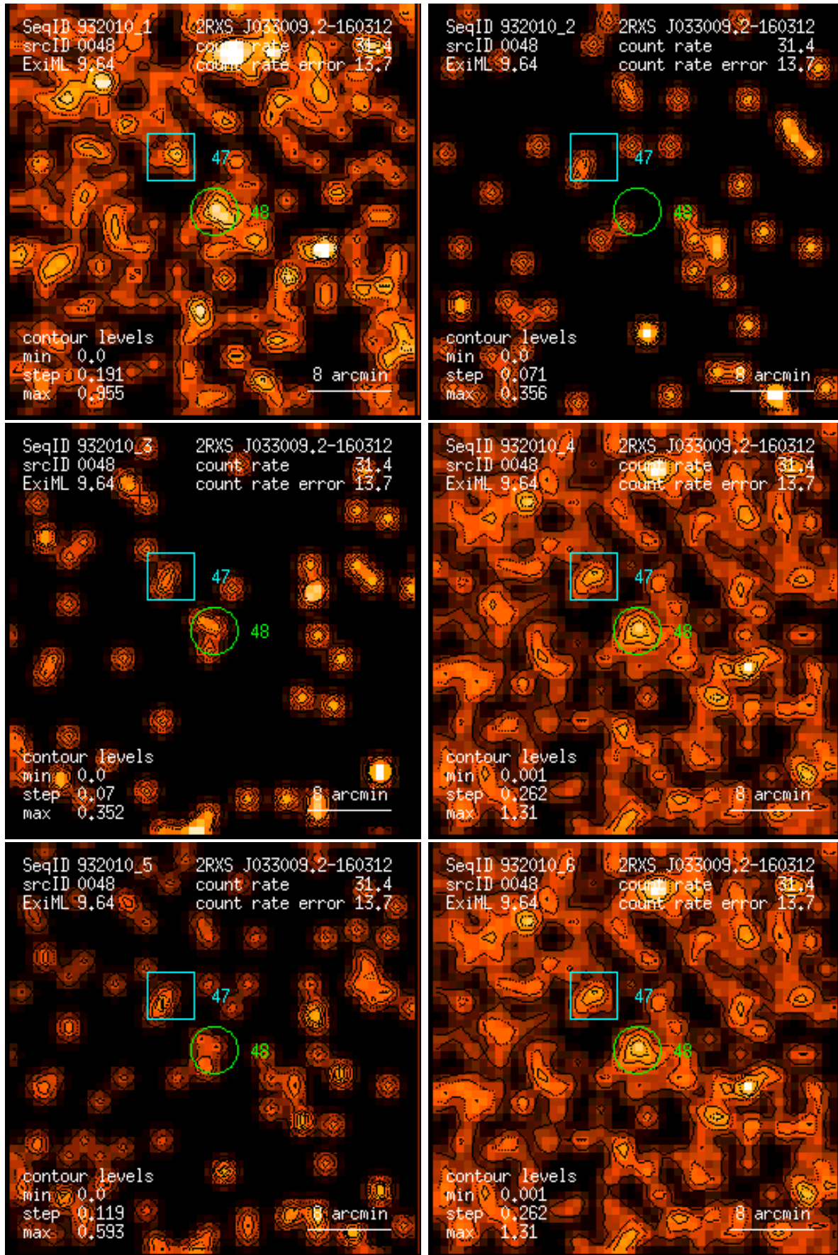
Figure 48: RASS 932010: detection 0048: band rate images, Gaussian filter: (1) PSPC channels 11 – 41, (2) 52 – 90, (3) 91 – 201, (4) 11 – 235, (5) 52 – 201, (6) 11 – 201. Broad band rates in counts/ks. Band rate contour levels in counts/ks/arcmin 2 .
