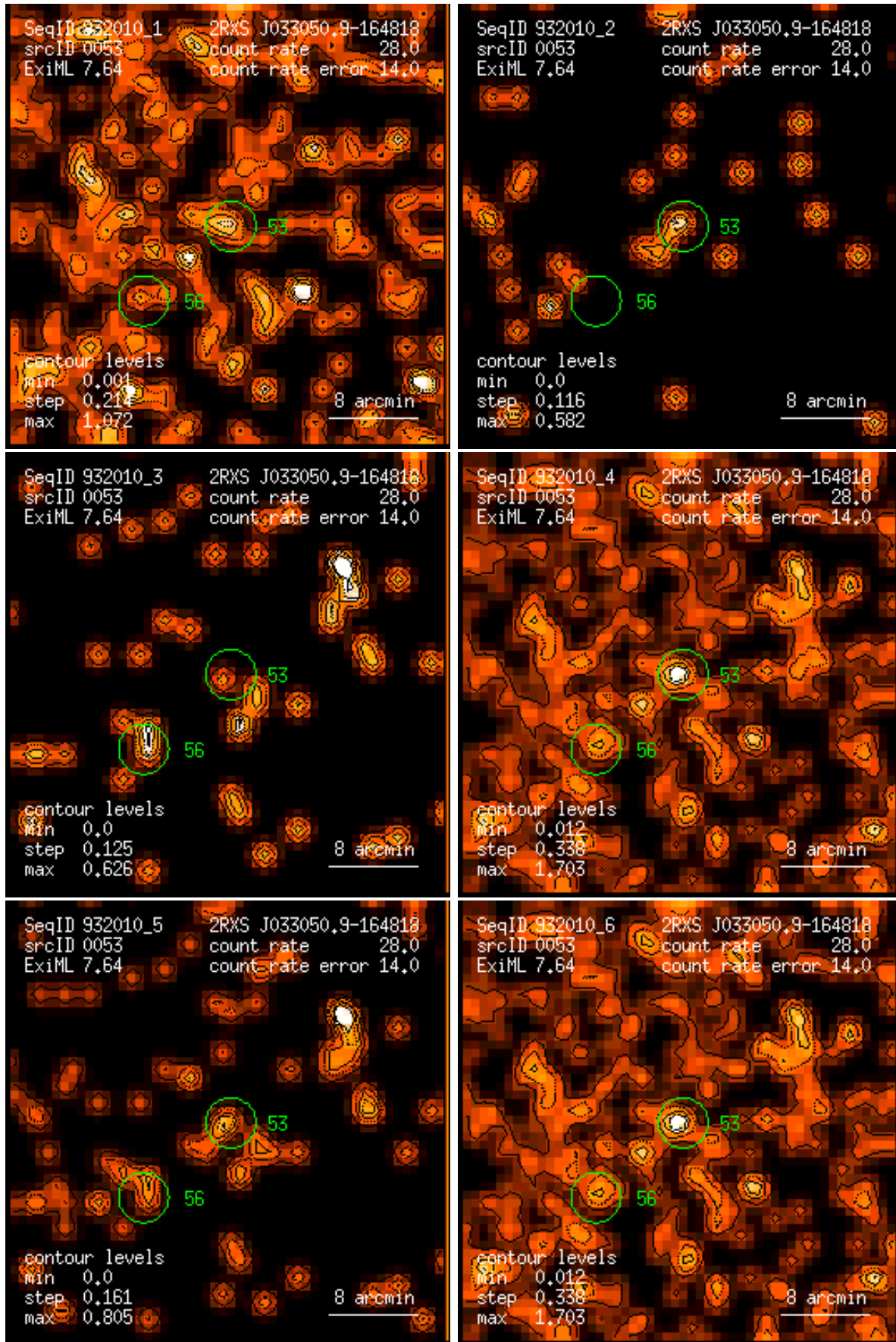
Figure 53: RASS 932010: detection 0053: band rate images, Gaussian filter: (1) PSPC channels 11 – 41, (2) 52 – 90, (3) 91 – 201, (4) 11 – 235, (5) 52 – 201, (6) 11 – 201. Broad band rates in counts/ks. Band rate contour levels in counts/ks/arcmin 2 .
