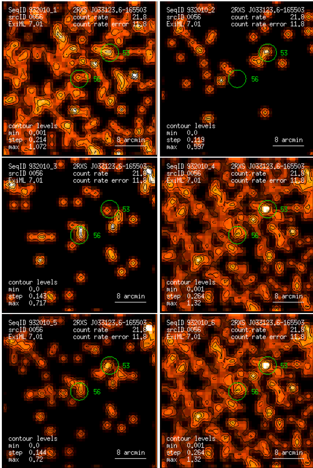
Figure 56: RASS 932010: detection 0056: band rate images, Gaussian filter: (1) PSPC channels 11 – 41, (2) 52 – 90, (3) 91 – 201, (4) 11 – 235, (5) 52 – 201, (6) 11 – 201. Broad band rates in counts/ks. Band rate contour levels in counts/ks/arcmin 2 .
