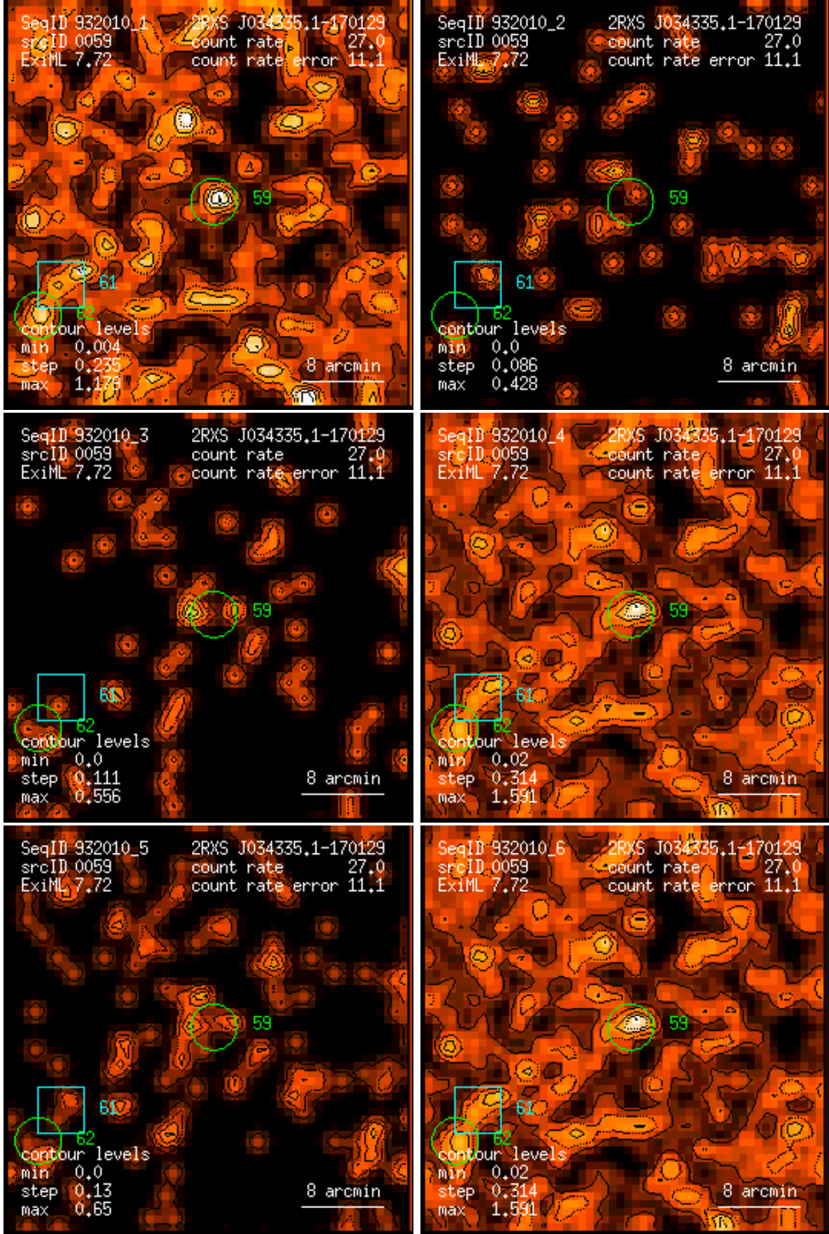
Figure 59: RASS 932010: detection 0059: band rate images, Gaussian filter: (1) PSPC channels 11 – 41, (2) 52 – 90, (3) 91 – 201, (4) 11 – 235, (5) 52 – 201, (6) 11 – 201. Broad band rates in counts/ks. Band rate contour levels in counts/ks/arcmin 2 .
