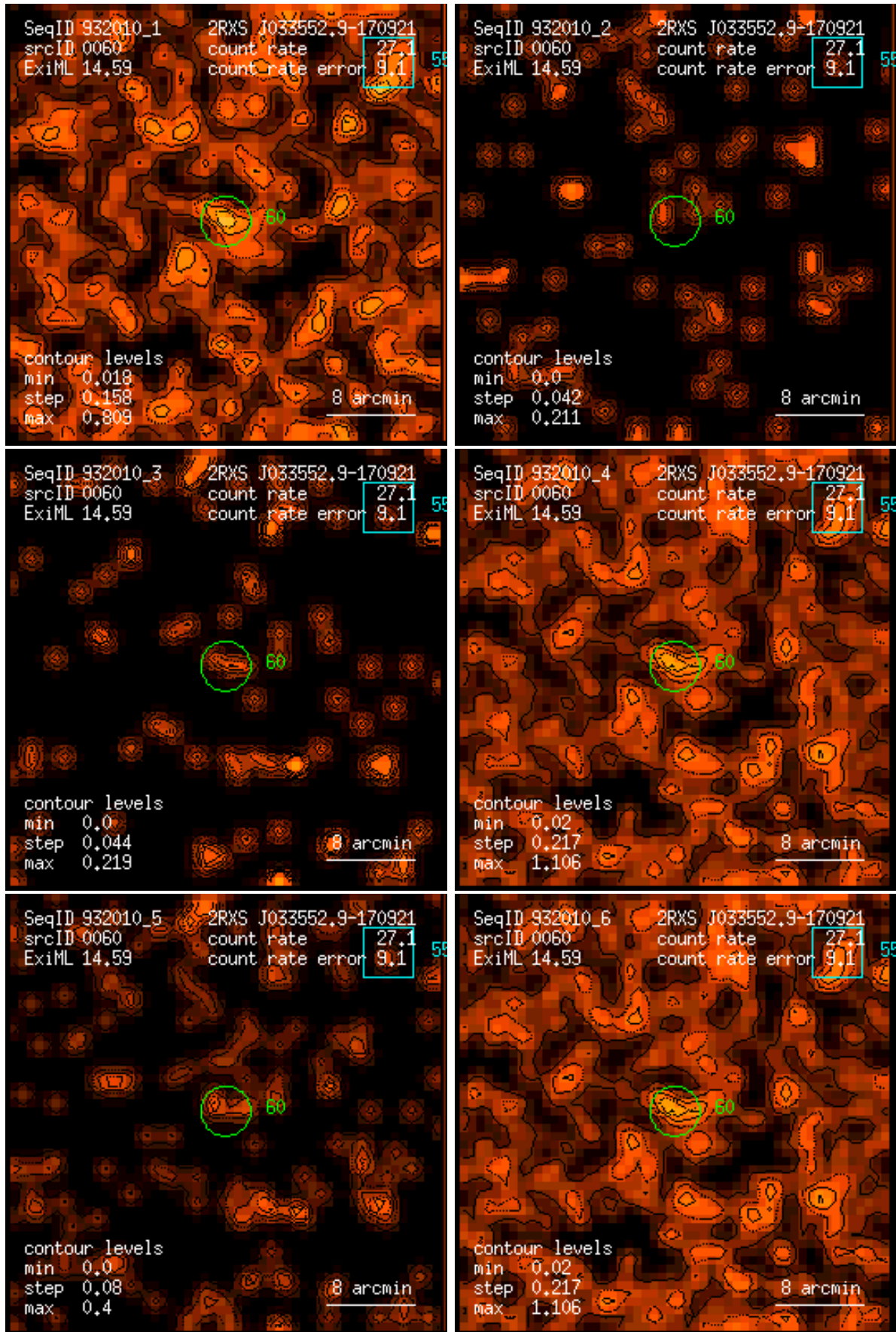
Figure 60: RASS 932010: detection 0060: band rate images, Gaussian filter: (1) PSPC channels 11 – 41, (2) 52 – 90, (3) 91 – 201, (4) 11 – 235, (5) 52 – 201, (6) 11 – 201. Broad band rates in counts/ks. Band rate contour levels in counts/ks/arcmin 2 .
