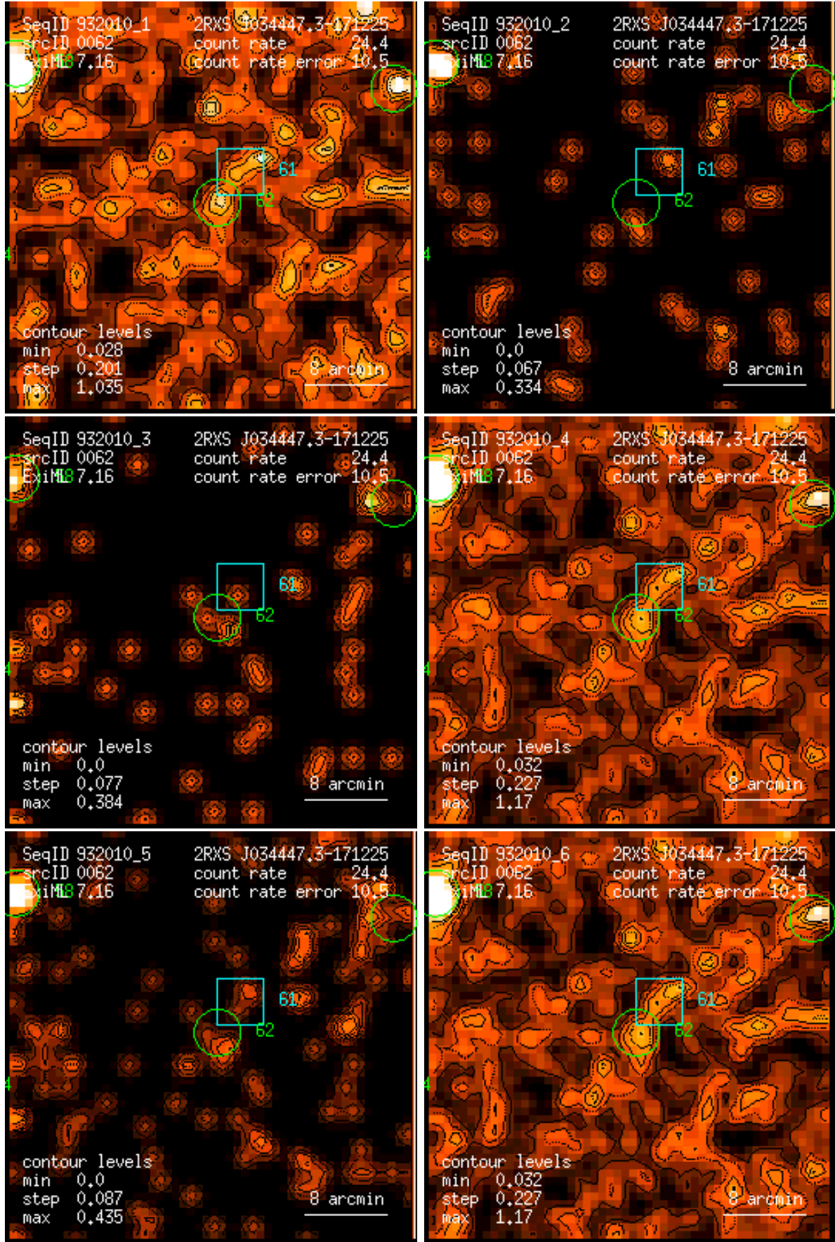
Figure 62: RASS 932010: detection 0062: band rate images, Gaussian filter: (1) PSPC channels 11 – 41, (2) 52 – 90, (3) 91 – 201, (4) 11 – 235, (5) 52 – 201, (6) 11 – 201. Broad band rates in counts/ks. Band rate contour levels in counts/ks/arcmin 2 .
