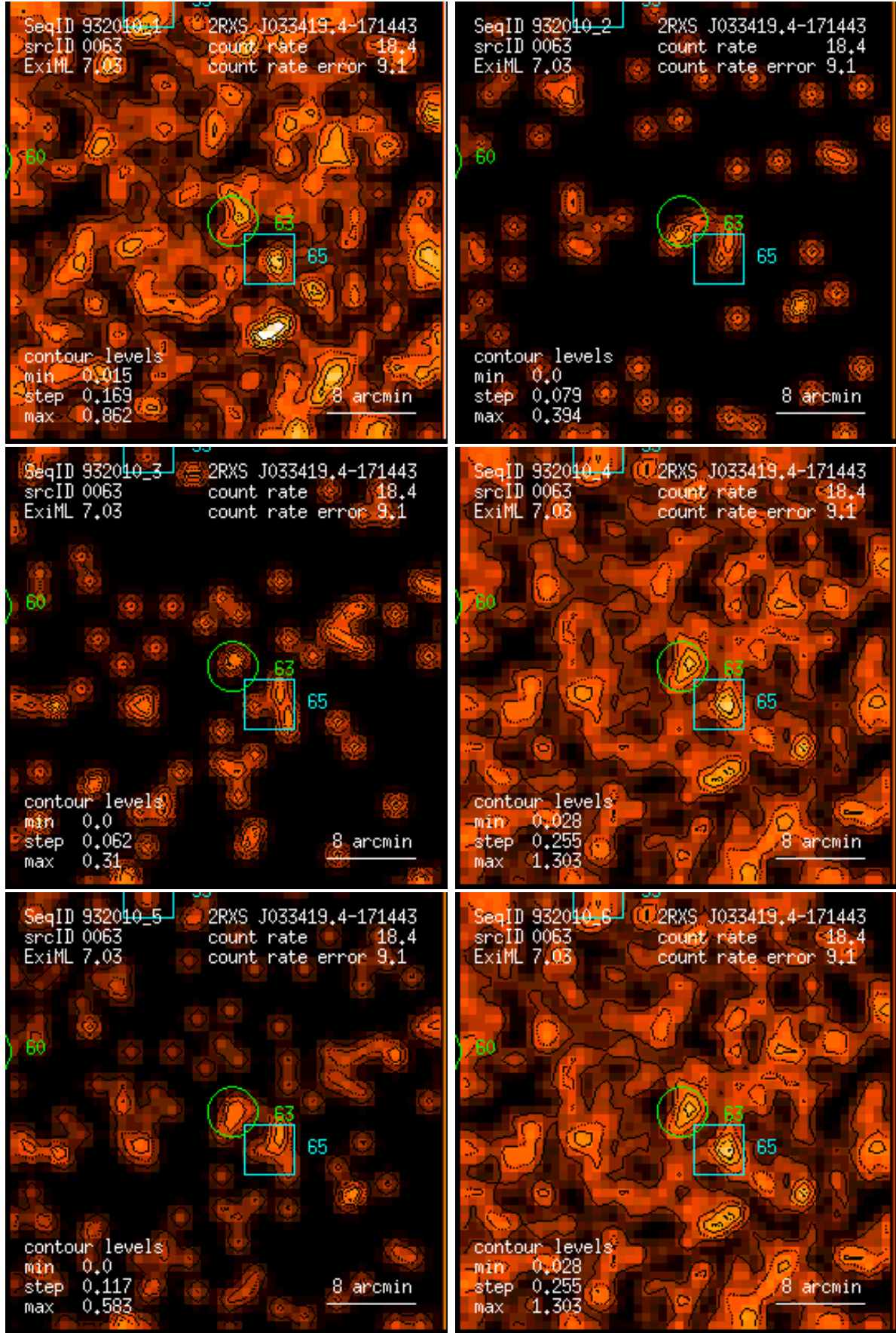
Figure 63: RASS 932010: detection 0063: band rate images, Gaussian filter: (1) PSPC channels 11 – 41, (2) 52 – 90, (3) 91 – 201, (4) 11 – 235, (5) 52 – 201, (6) 11 – 201. Broad band rates in counts/ks. Band rate contour levels in counts/ks/arcmin 2 .
