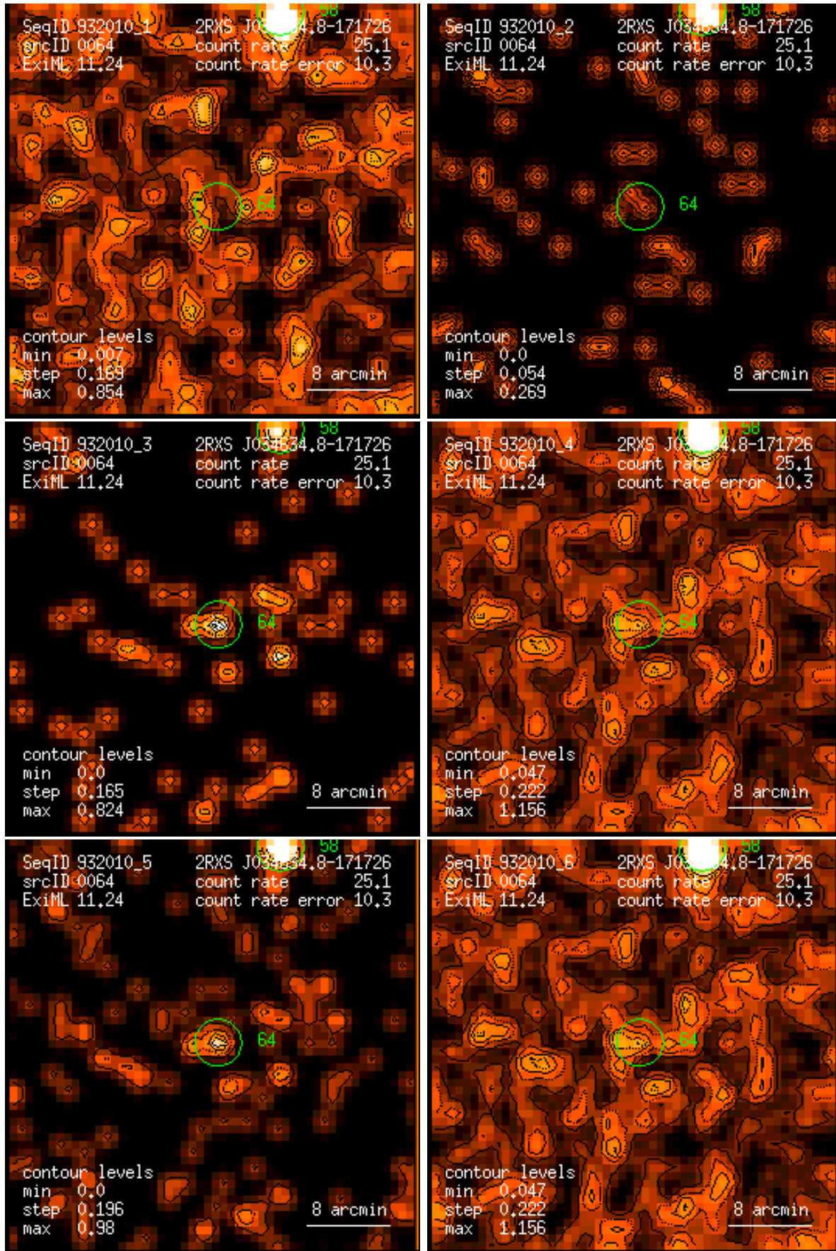
Figure 64: RASS 932010: detection 0064: band rate images, Gaussian filter: (1) PSPC channels 11 – 41, (2) 52 – 90, (3) 91 – 201, (4) 11 – 235, (5) 52 – 201, (6) 11 – 201. Broad band rates in counts/ks. Band rate contour levels in counts/ks/arcmin 2 .
