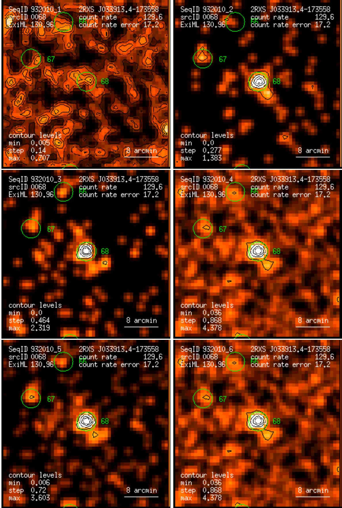
Figure 68: RASS 932010: detection 0068: band rate images, Gaussian filter: (1) PSPC channels 11 – 41, (2) 52 – 90, (3) 91 – 201, (4) 11 – 235, (5) 52 – 201, (6) 11 – 201. Broad band rates in counts/ks. Band rate contour levels in counts/ks/arcmin 2 .
