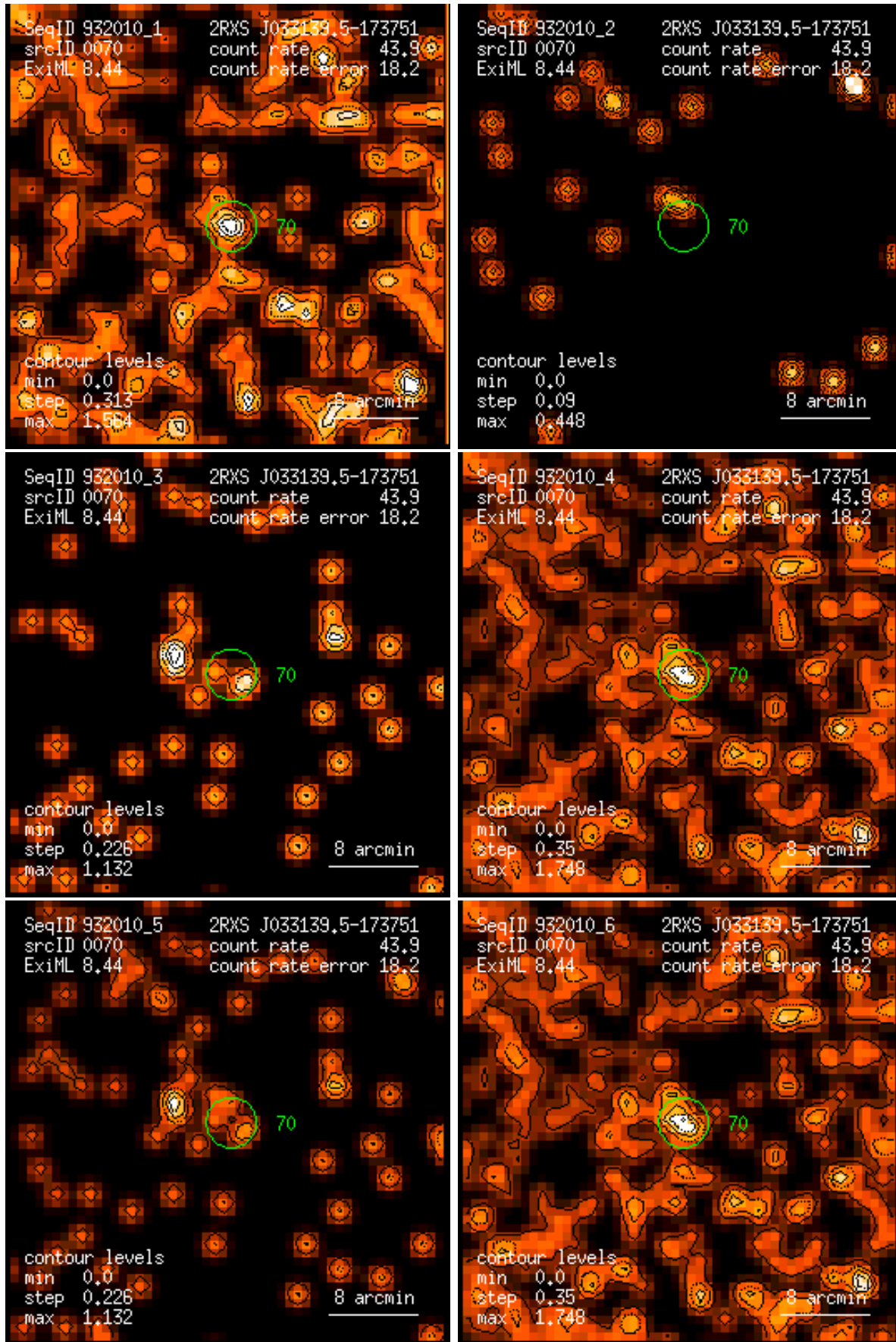
Figure 70: RASS 932010: detection 0070: band rate images, Gaussian filter: (1) PSPC channels 11 – 41, (2) 52 – 90, (3) 91 – 201, (4) 11 – 235, (5) 52 – 201, (6) 11 – 201. Broad band rates in counts/ks. Band rate contour levels in counts/ks/arcmin 2 .
