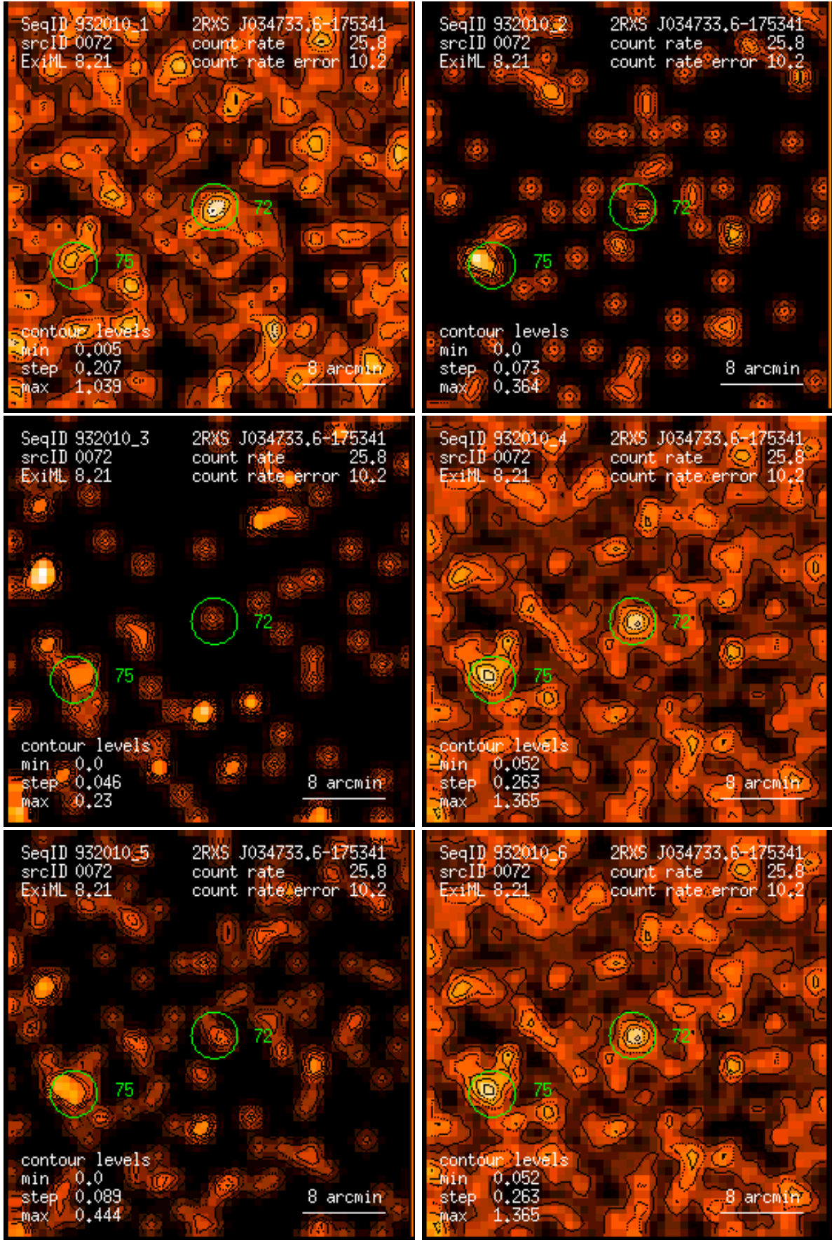
Figure 72: RASS 932010: detection 0072: band rate images, Gaussian filter: (1) PSPC channels 11 – 41, (2) 52 – 90, (3) 91 – 201, (4) 11 – 235, (5) 52 – 201, (6) 11 – 201. Broad band rates in counts/ks. Band rate contour levels in counts/ks/arcmin 2 .
