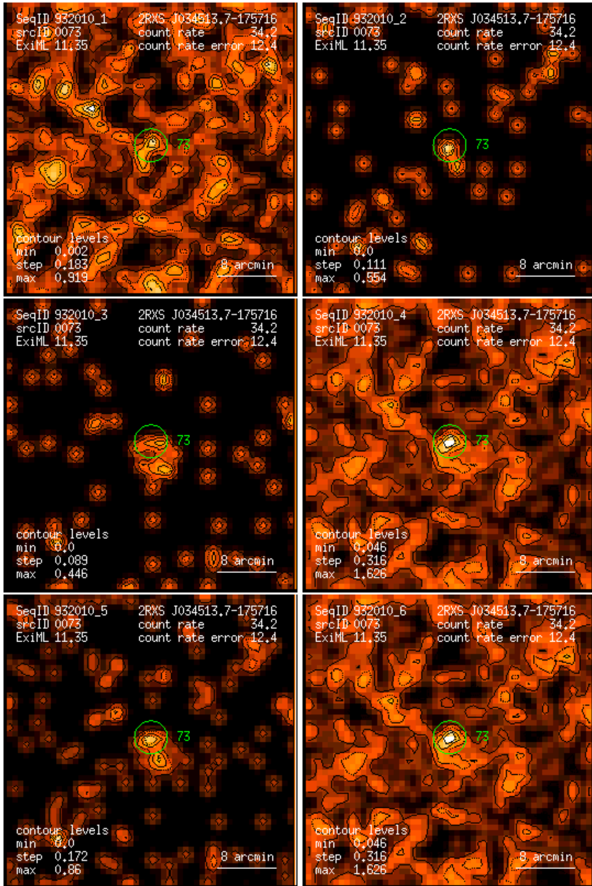
Figure 73: RASS 932010: detection 0073: band rate images, Gaussian filter: (1) PSPC channels 11 – 41, (2) 52 – 90, (3) 91 – 201, (4) 11 – 235, (5) 52 – 201, (6) 11 – 201. Broad band rates in counts/ks. Band rate contour levels in counts/ks/arcmin 2 .
