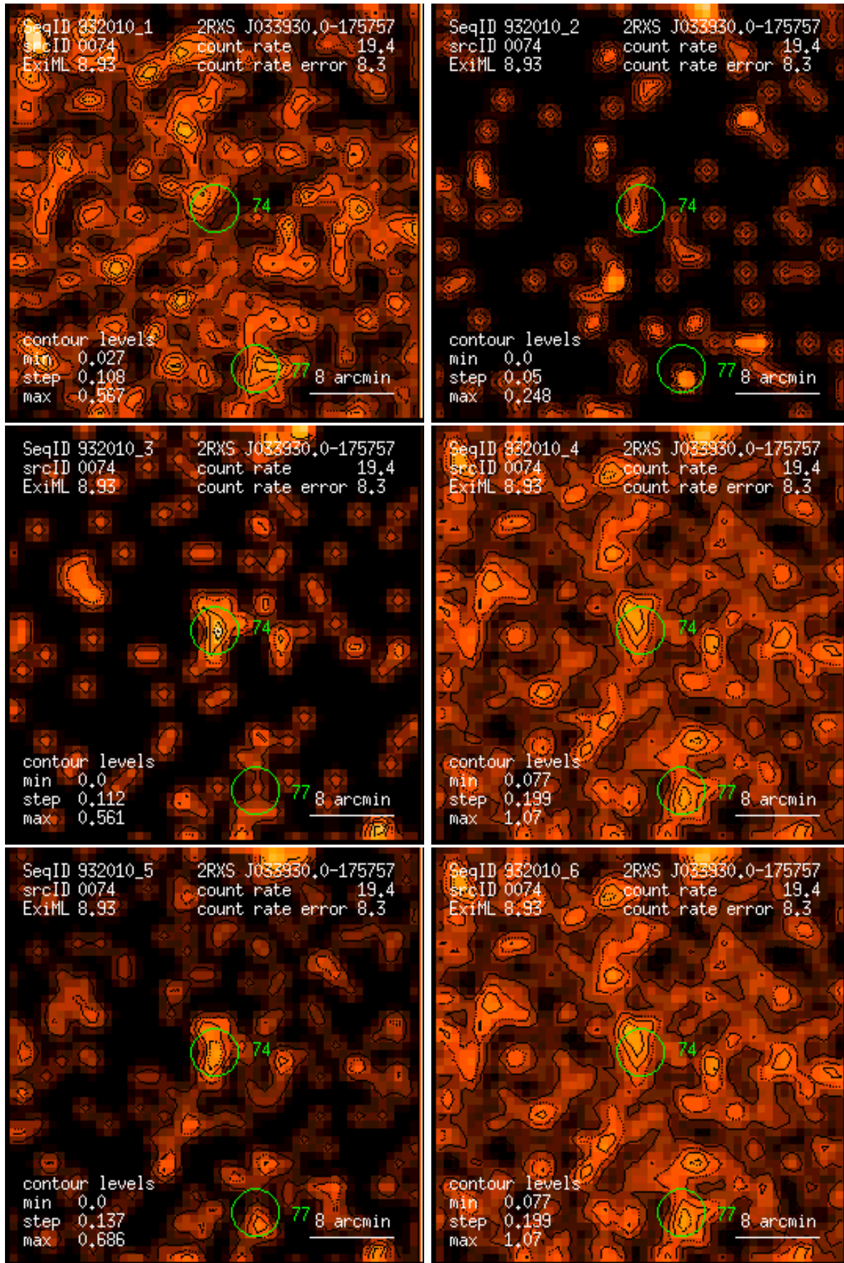
Figure 74: RASS 932010: detection 0074: band rate images, Gaussian filter: (1) PSPC channels 11 – 41, (2) 52 – 90, (3) 91 – 201, (4) 11 – 235, (5) 52 – 201, (6) 11 – 201. Broad band rates in counts/ks. Band rate contour levels in counts/ks/arcmin 2 .
